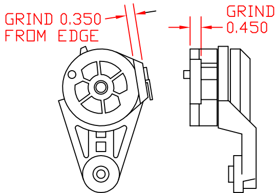
FIG. 7 OEM BELT TENSIONER
