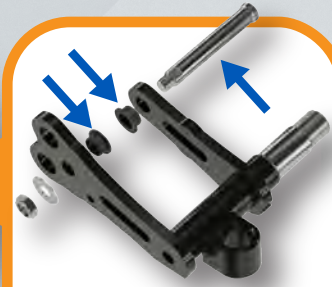
SPINDLE BUSHINGS & PIVOT PINS
