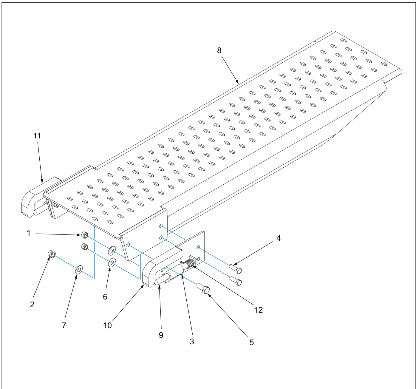
Figure 1-103: Front Slope
