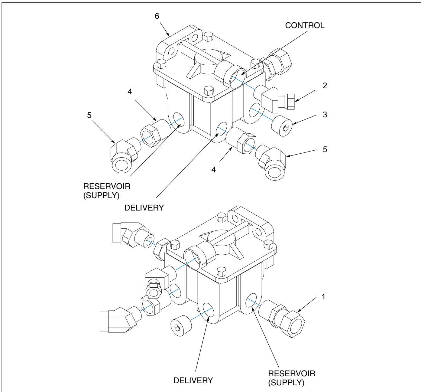
Figure 1-21: Valve Assembly - Air Booster
