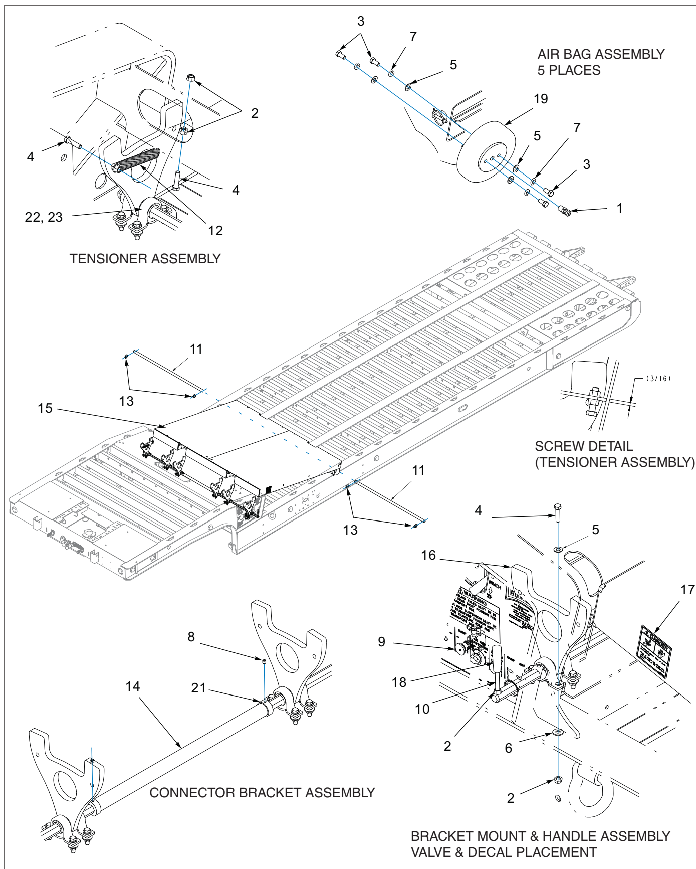
Figure 1-9: 6' Air Ramp - General Assembly
