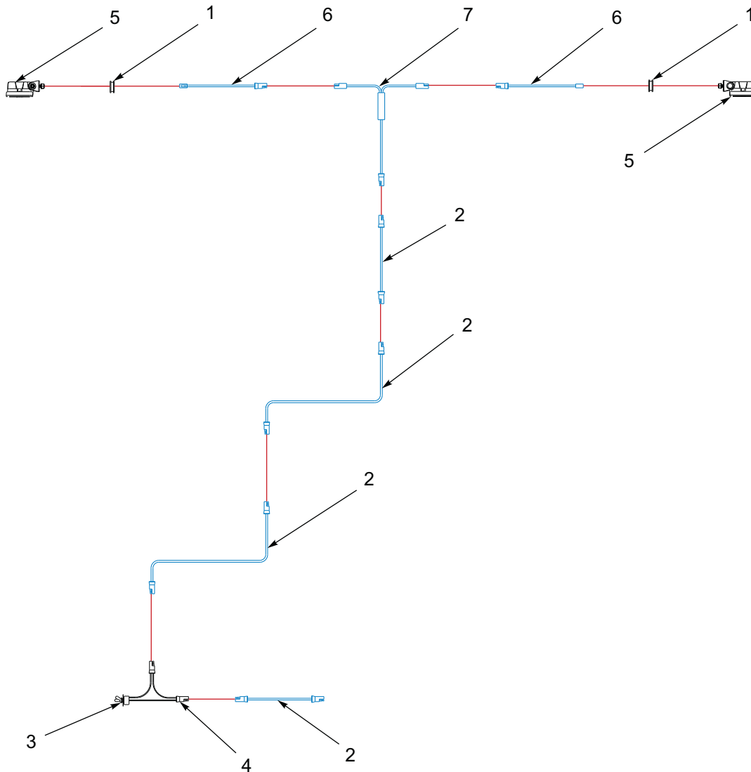
Figure 1-122: Work Light Installation
