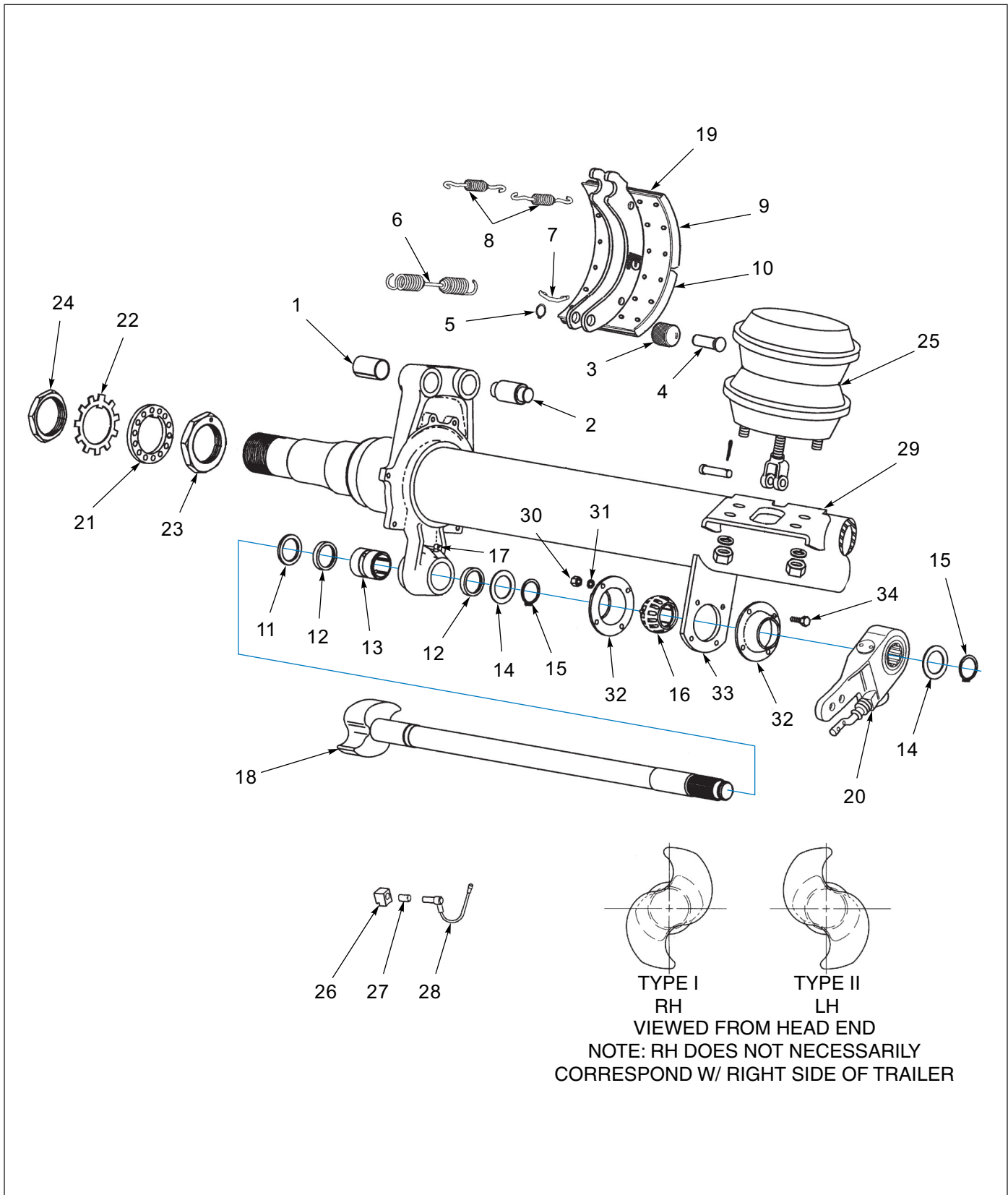
Figure 1-41: Dexter 12-1/4" X 7-1/2"
