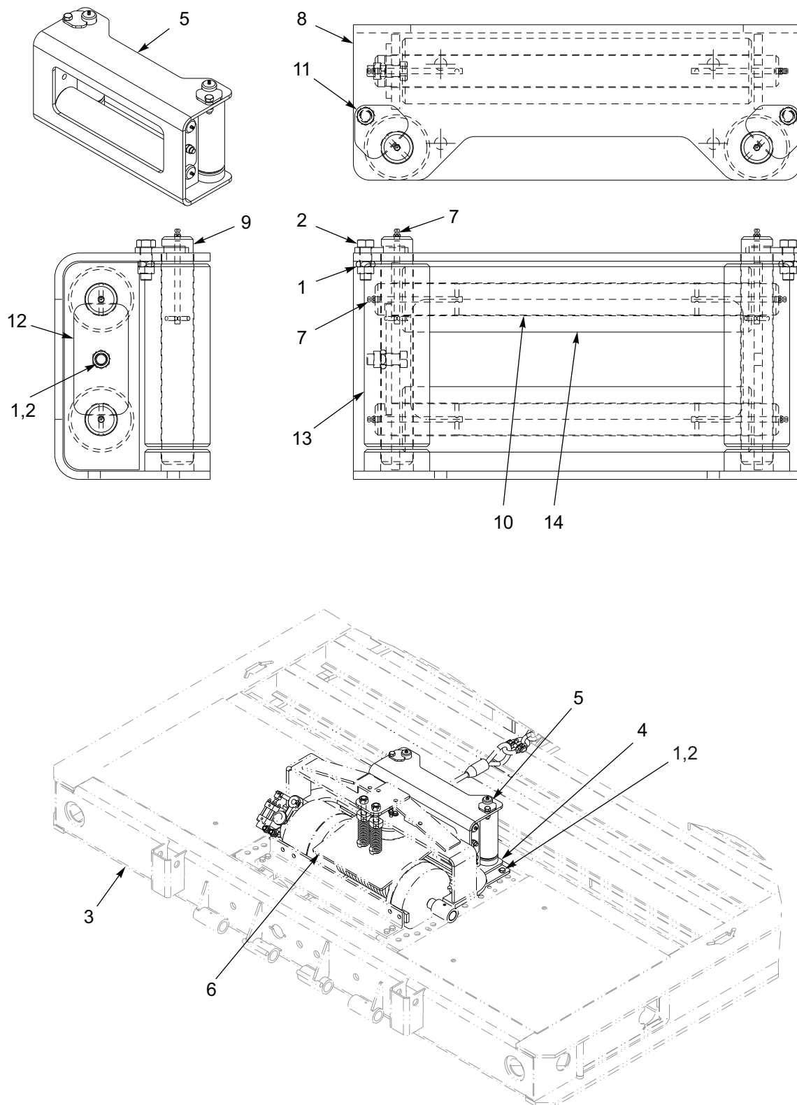
Figure 1-106: 4 Roller Guide Installation - 20K (BRADEN)
