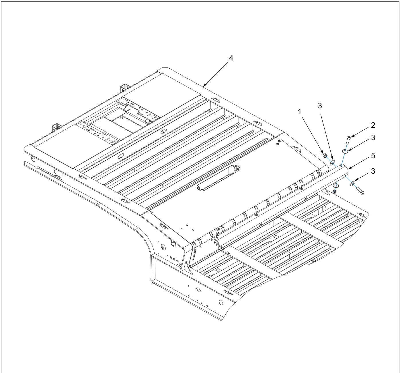
Figure 1-77: Fork Lift Plate Installation
