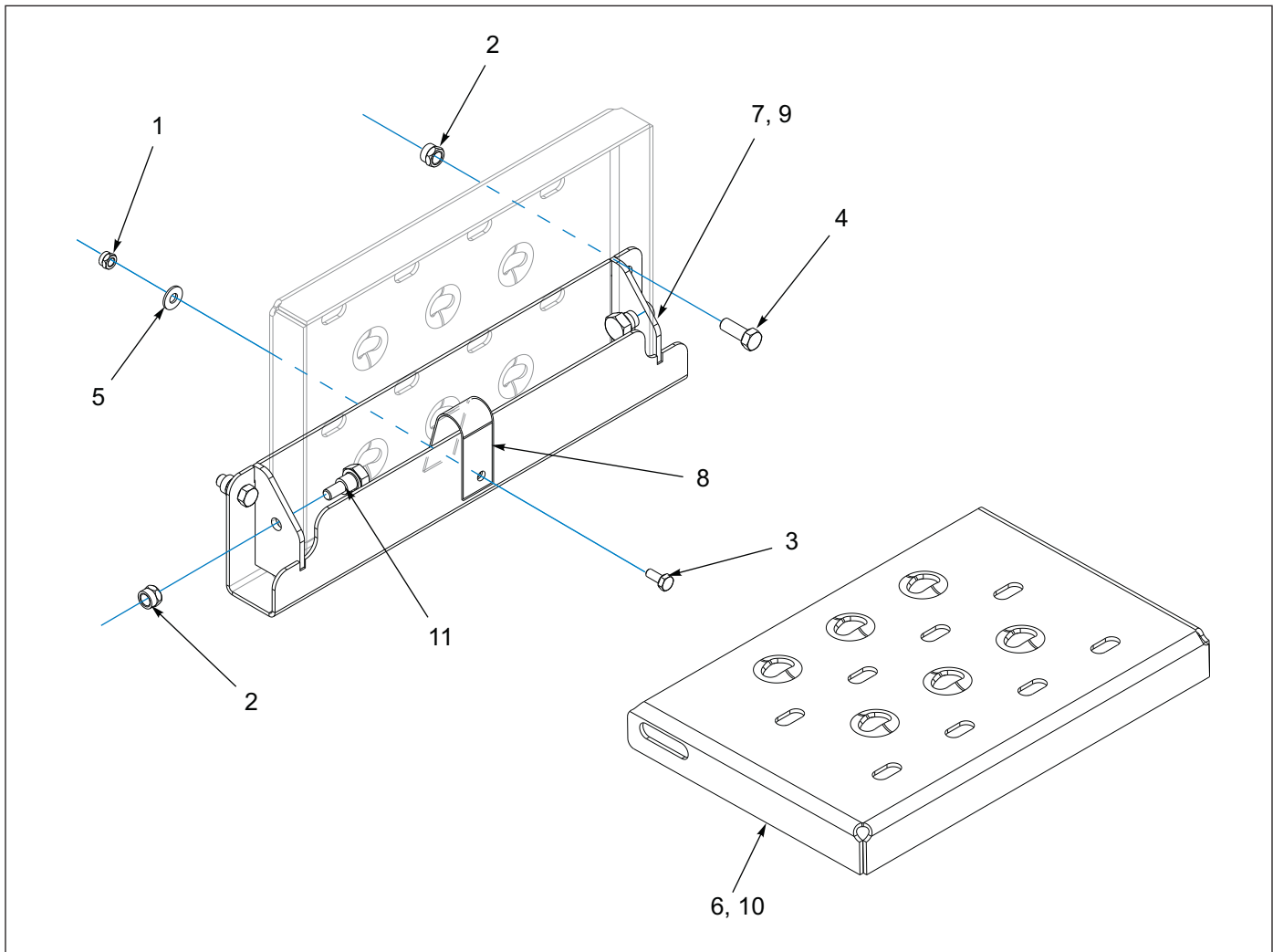
Figure 1-110: Folding Step Assembly - Double Drop Frame
