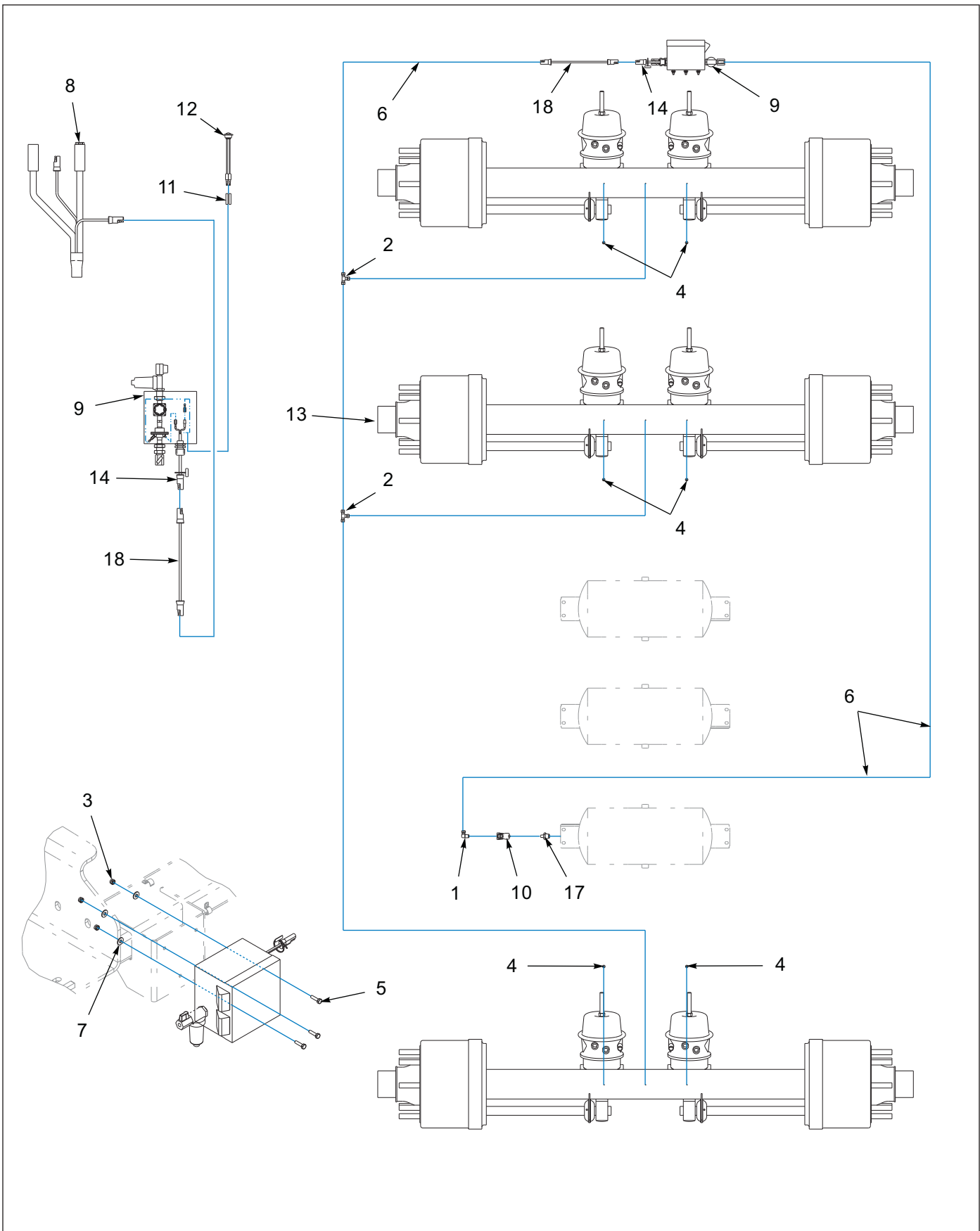
Figure 1-49: Tire Inflation System - 950E
