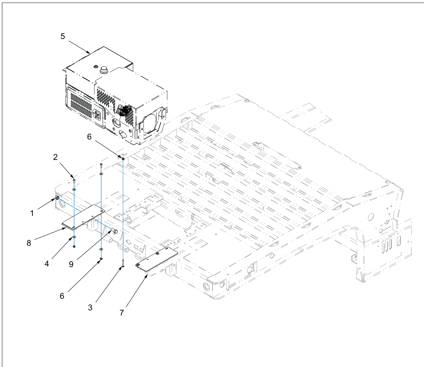
Figure 1-92: Front Mount Installation
