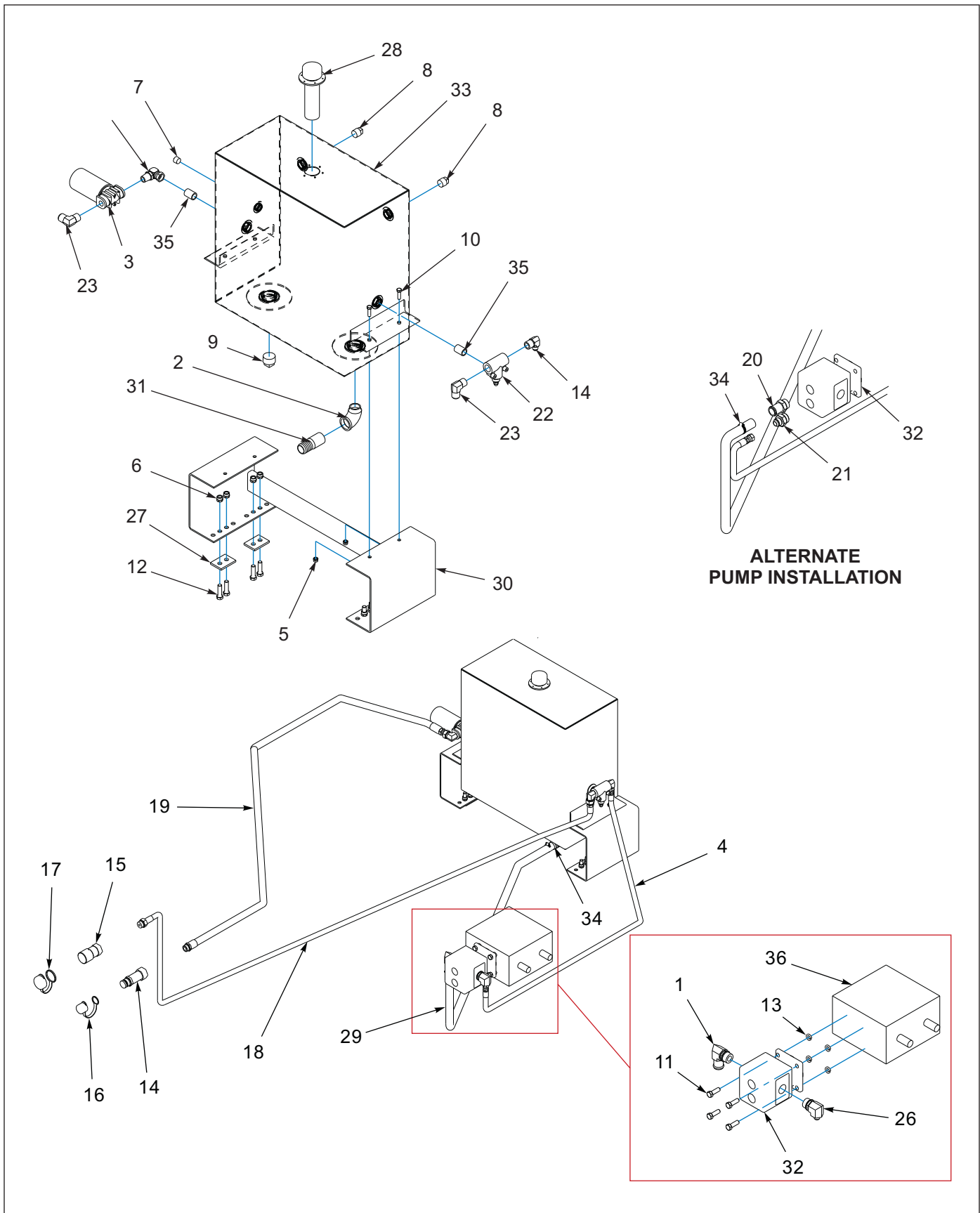
Figure 1-97: Hydraulic Wet Kit Items - 30 Gallon
