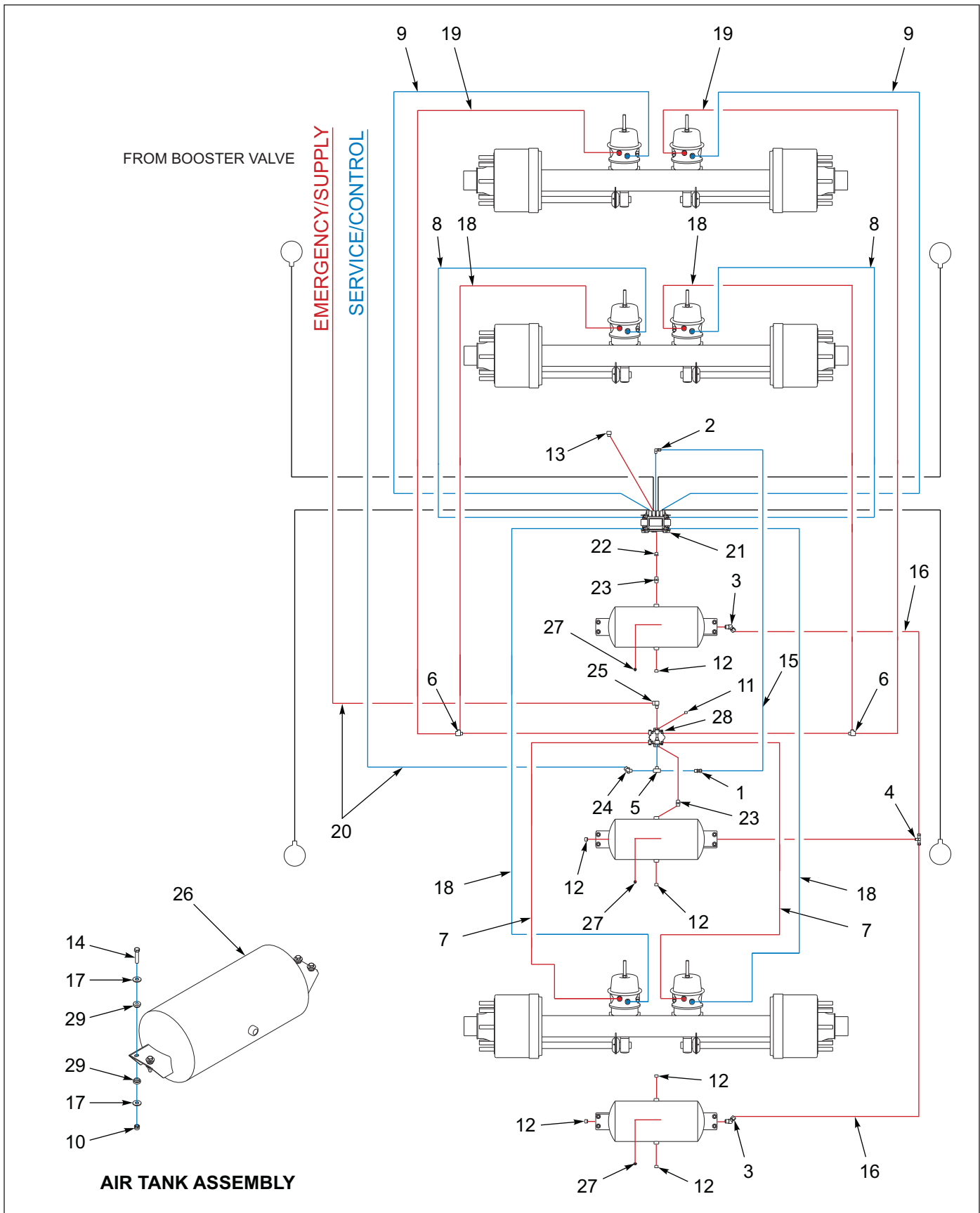
Figure 1-46: Air Brake System - 950E
