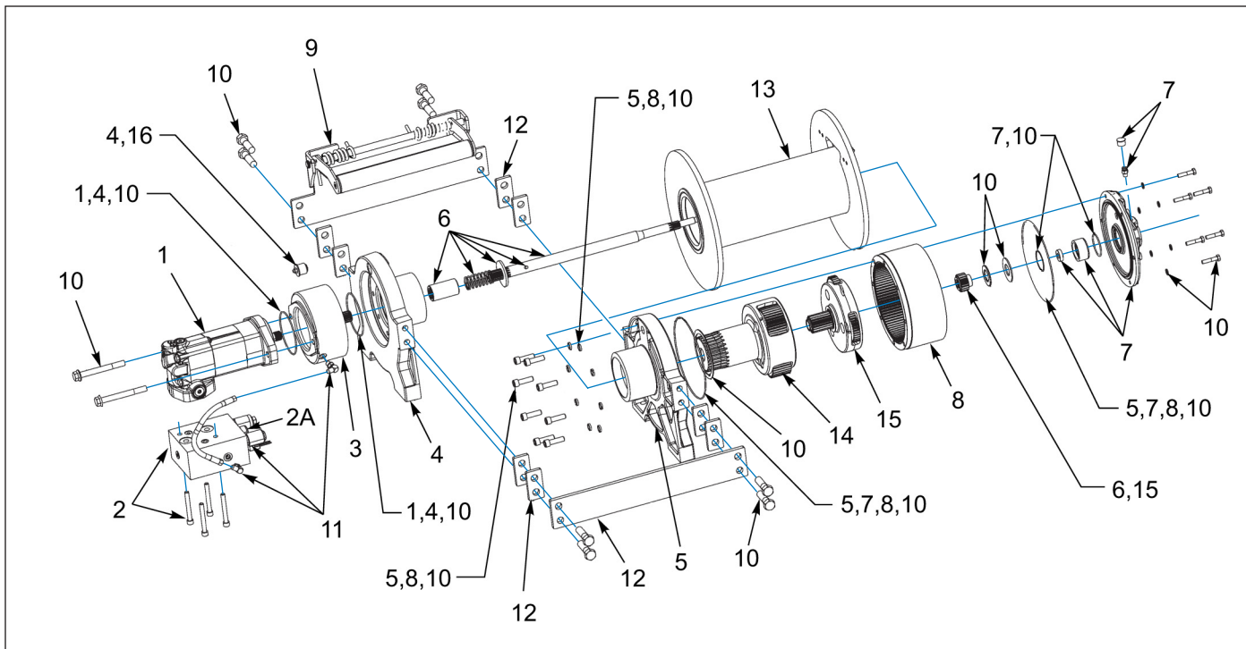
Figure 1-66: Winch Items - 30K 2 Speed (WARN)
