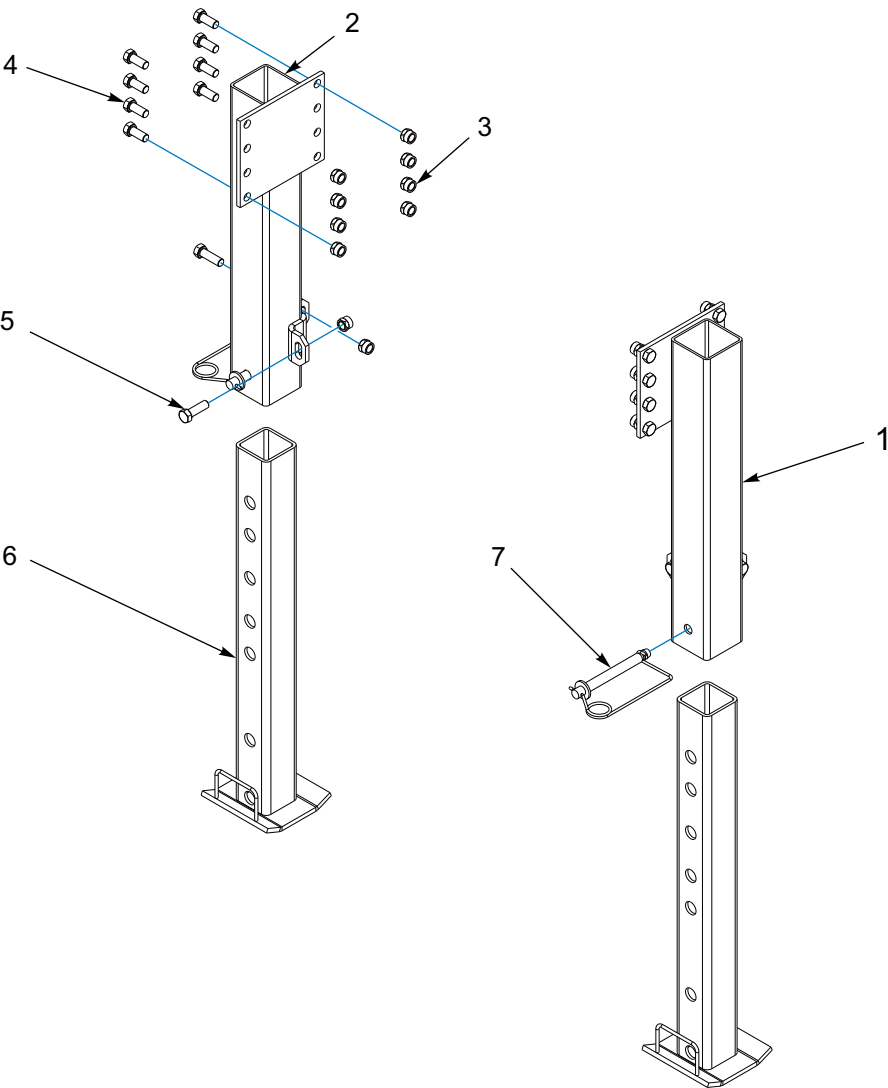
Figure 1-67: “Bolt On” Park Stand
