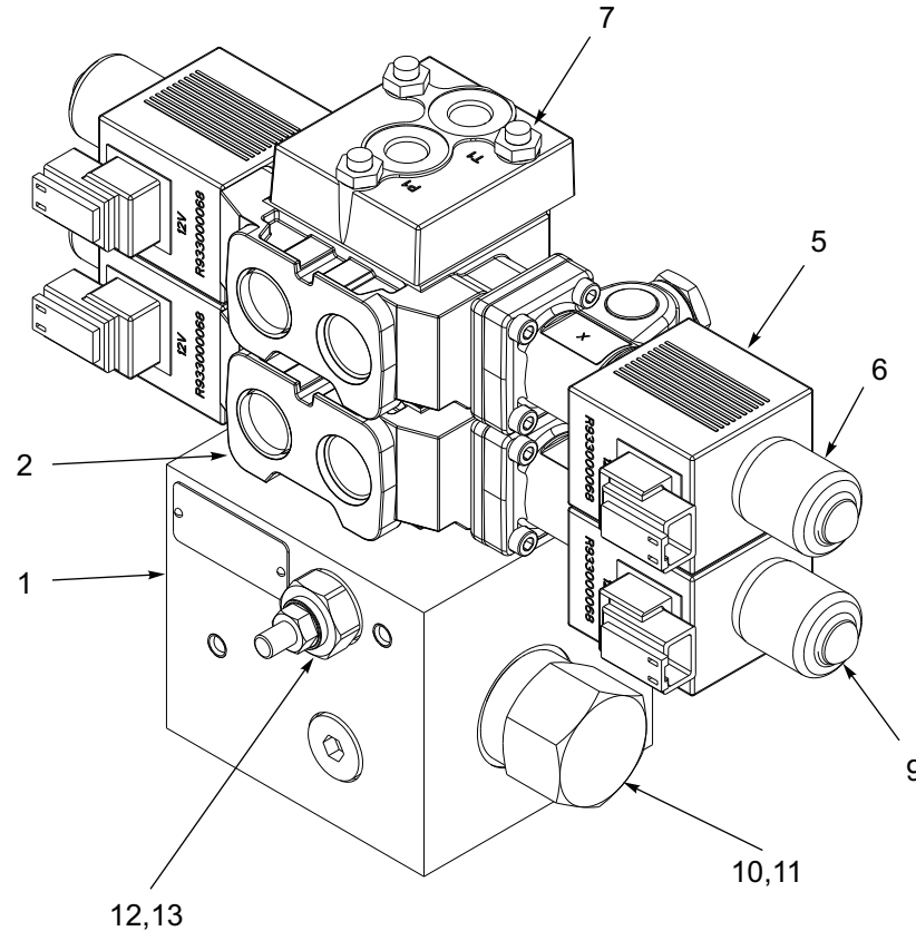
Figure 1-23: Valve Assembly - 2 Spool Solenoid
