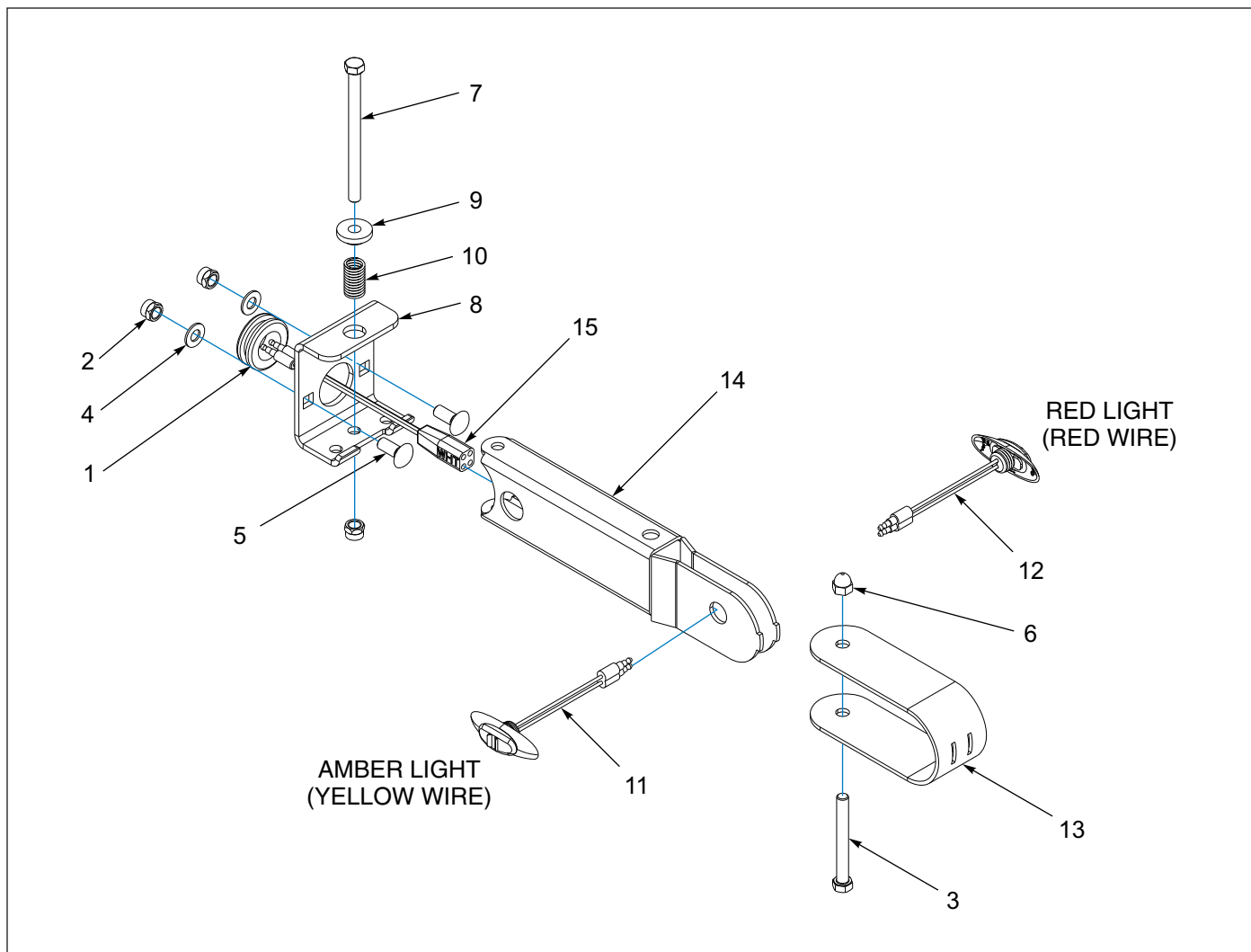
Figure 1-101: Swing-Arm Light Assembly - STREET
