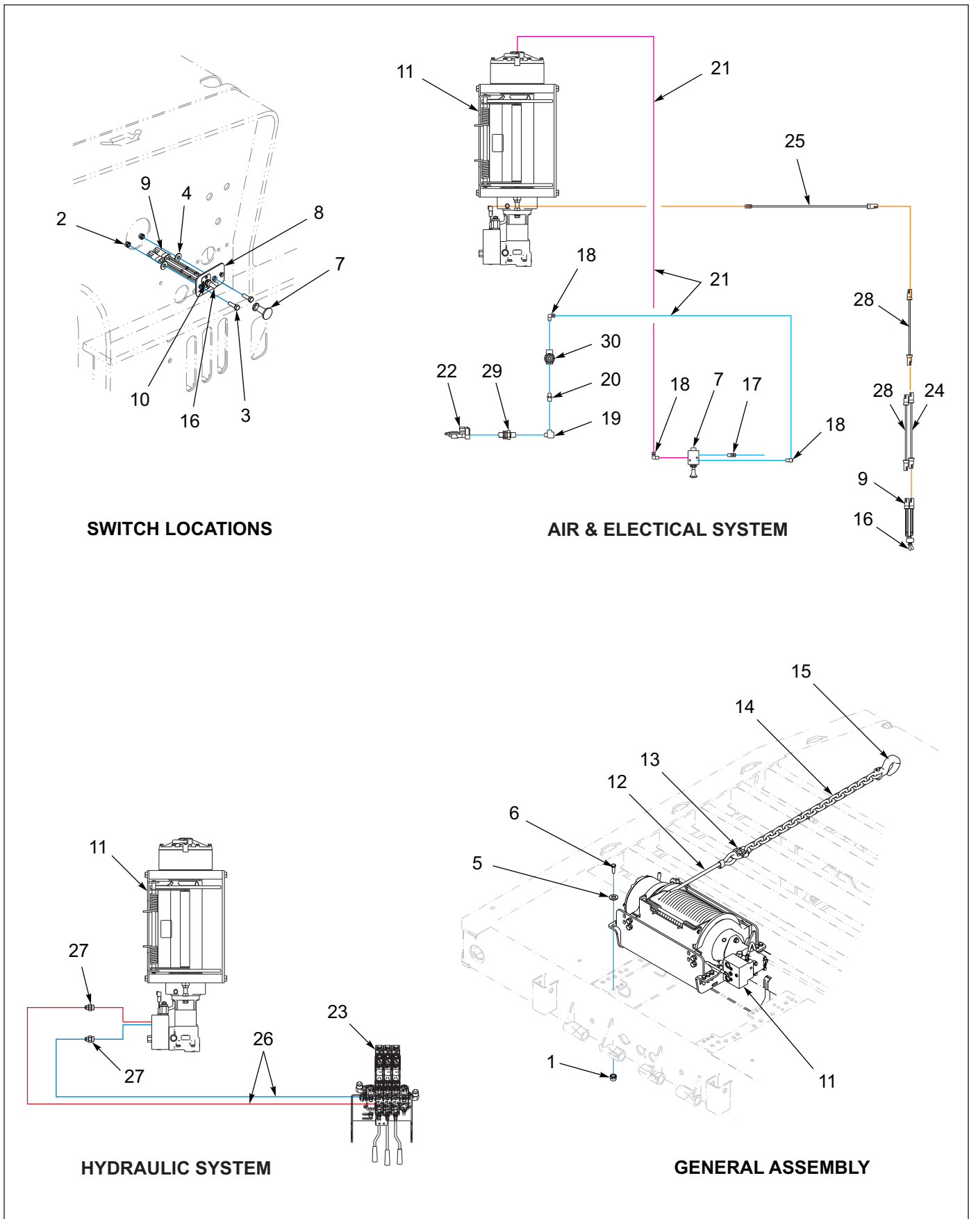
Figure 1-63: Winch Installation - 20K 2 Speed (WARN)
