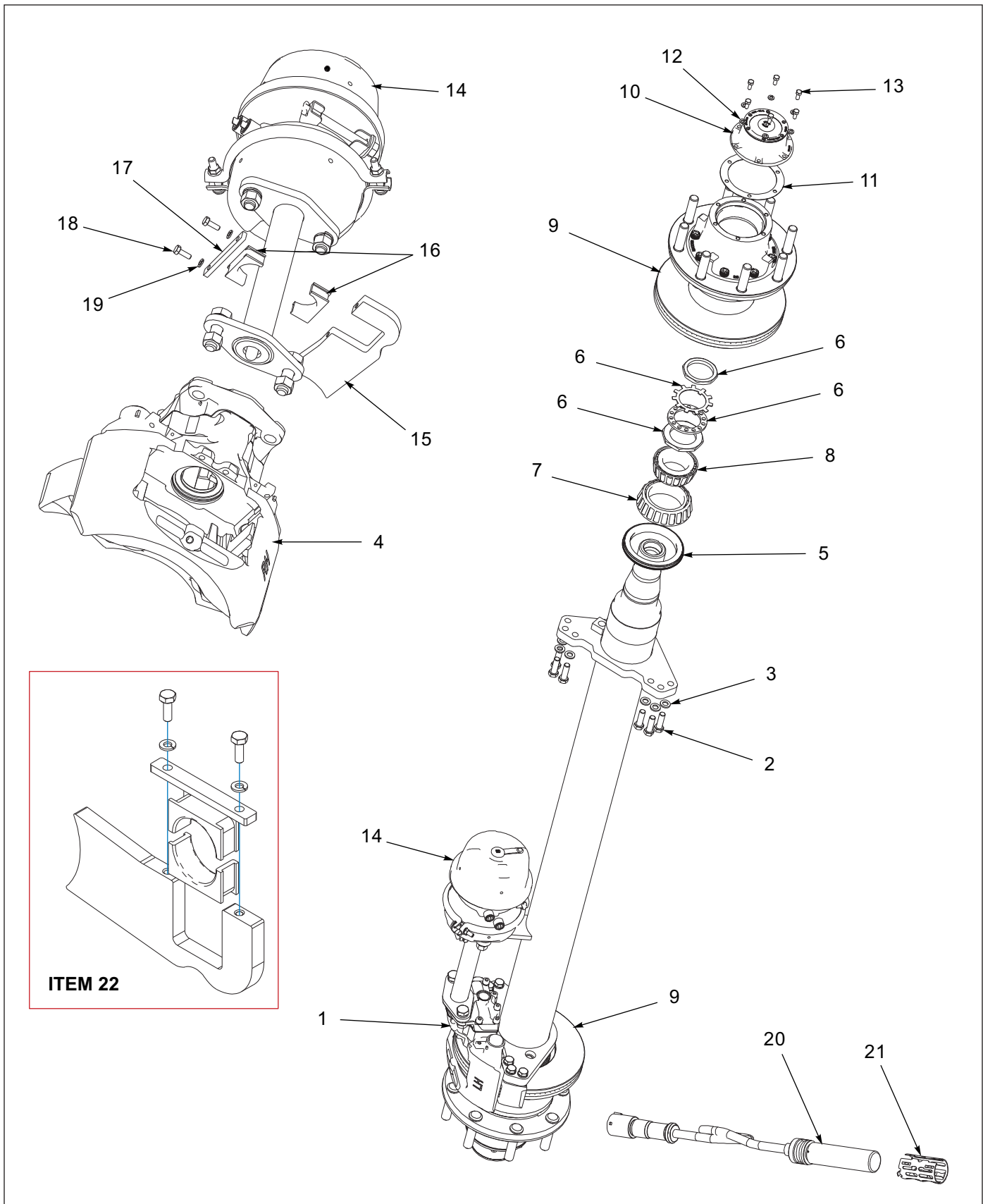
Figure 1-44: Dexter Disc Brakes
