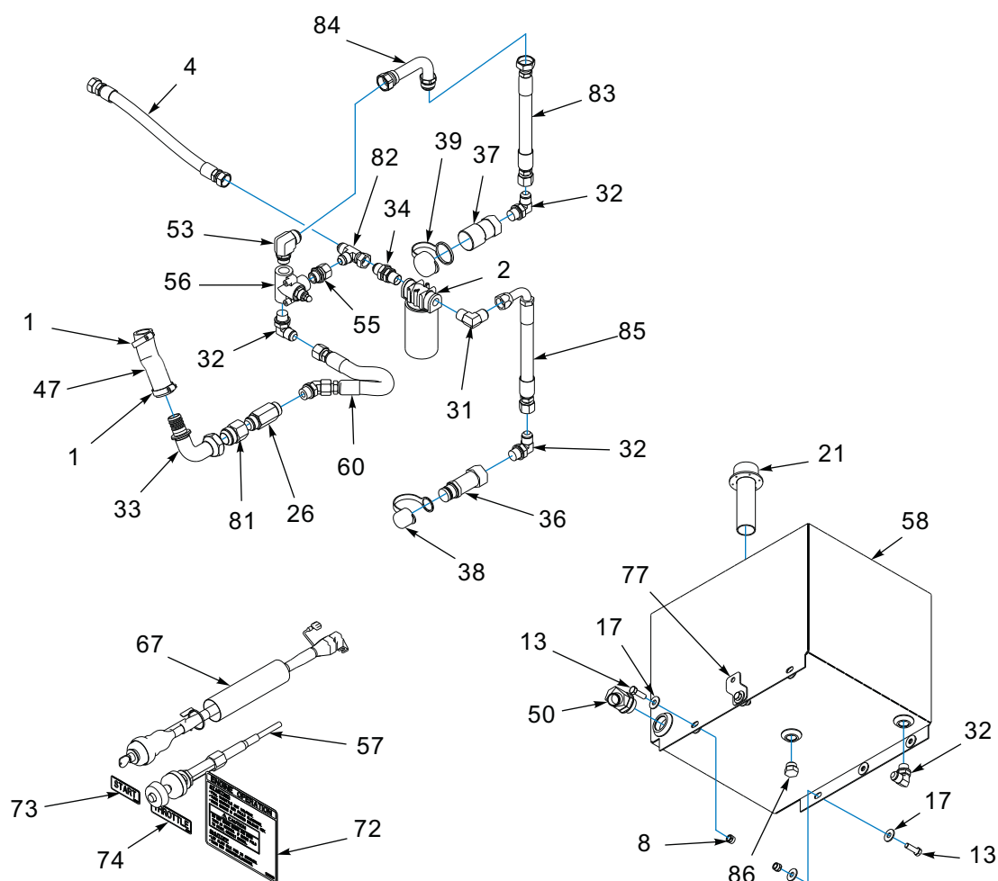
Figure 1-86: 25 HP Upper Deck Package (4 of 4)
