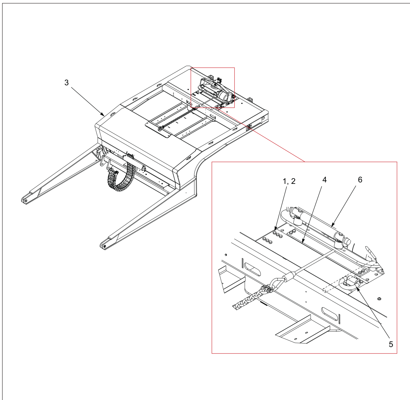
Figure 1-120: Trim Plate Installation
