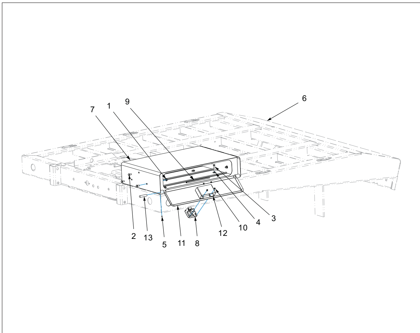
Figure 1-113: Toolbox Installation - Upper Deck
