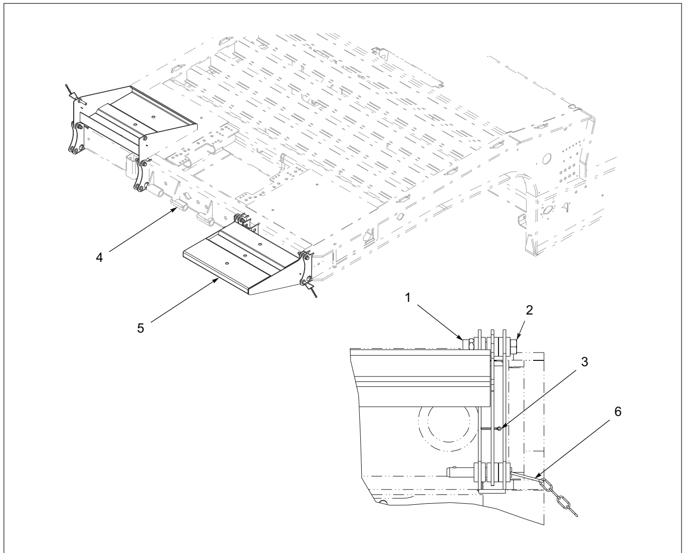
Figure 1-123: Front Flip Option
