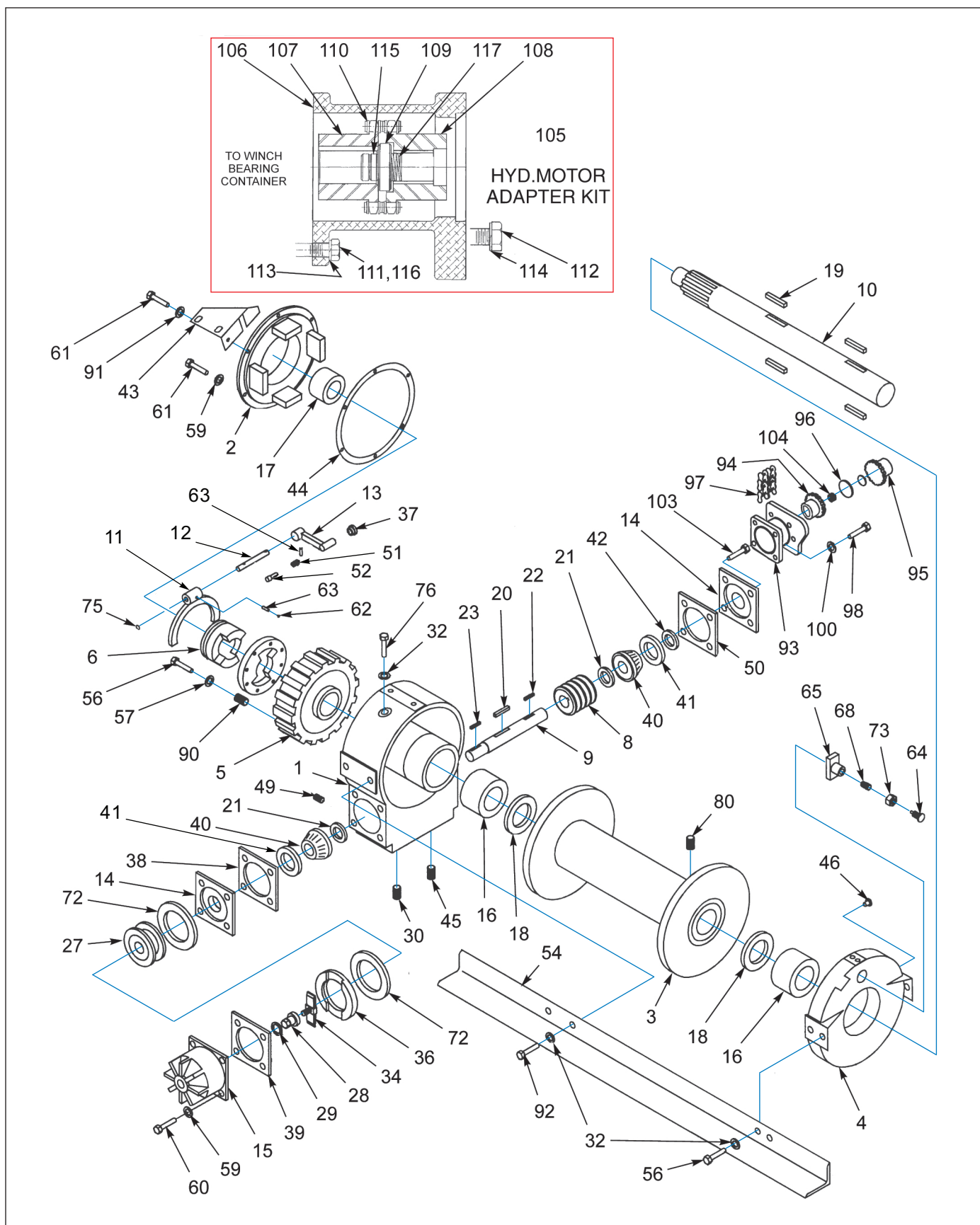
Figure 1-58: Winch Items - 20,000Lb. (BRADEN)
