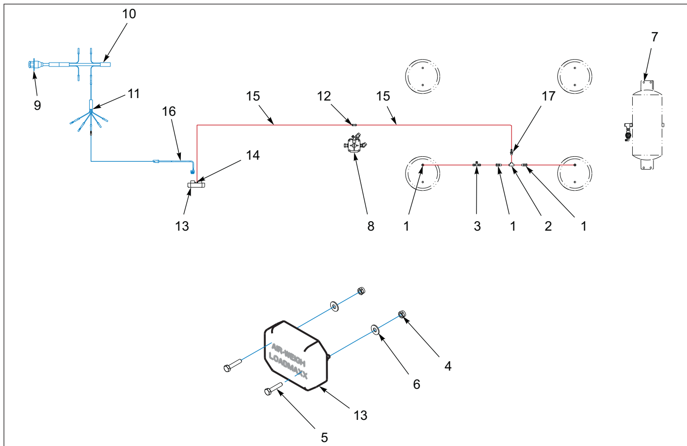
Figure 1-70: Loadmax System
