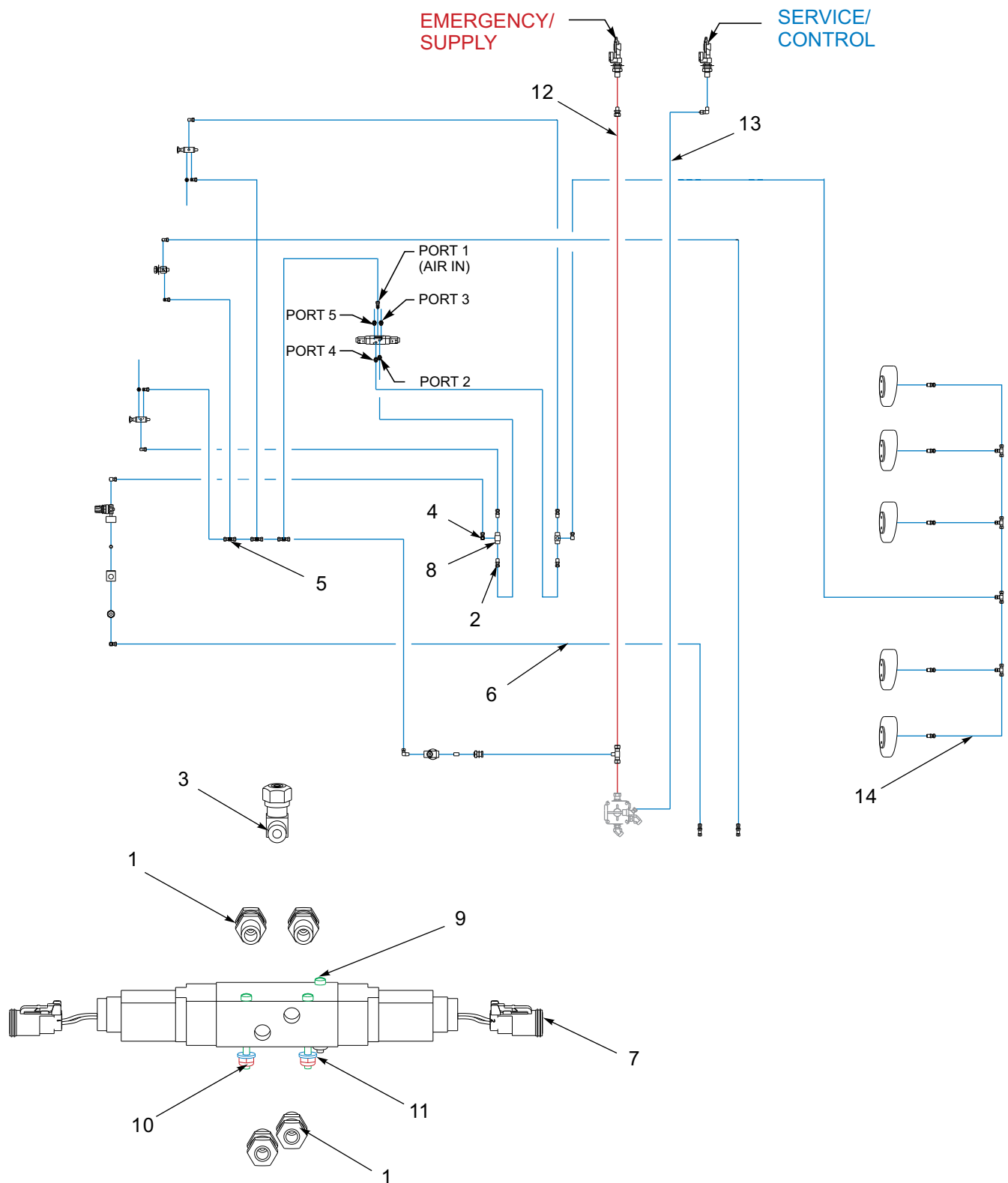
Figure 1-18: Ramp and Dock Lift Air Items
