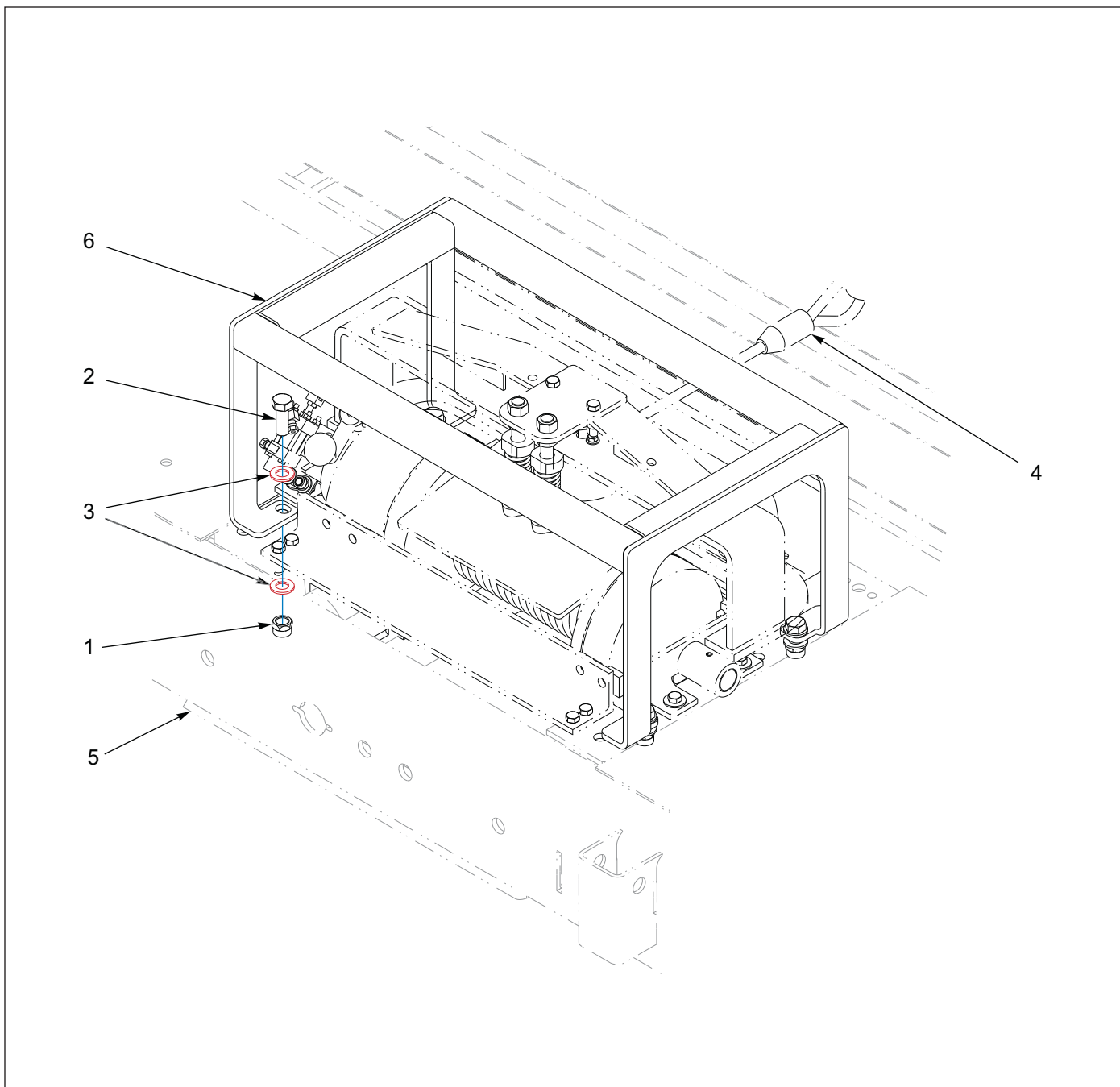
Figure 1-118: 20K Pivot Guard Installation
