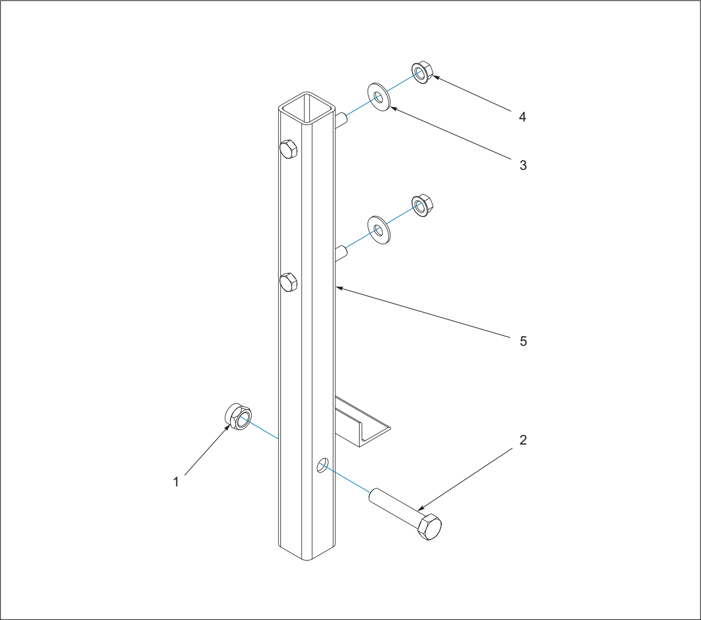
Figure 1-108: Spare Tire Mount Assembly
