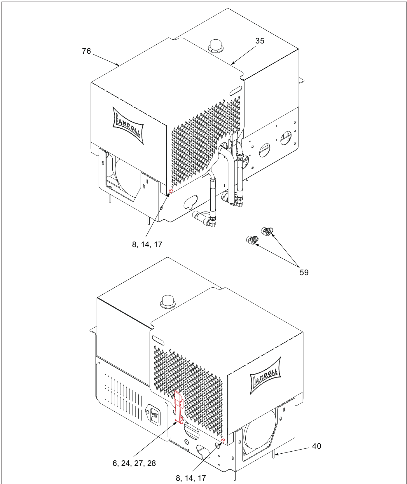
Figure 1-83: 25 HP Upper Deck Package (1 of 4)
