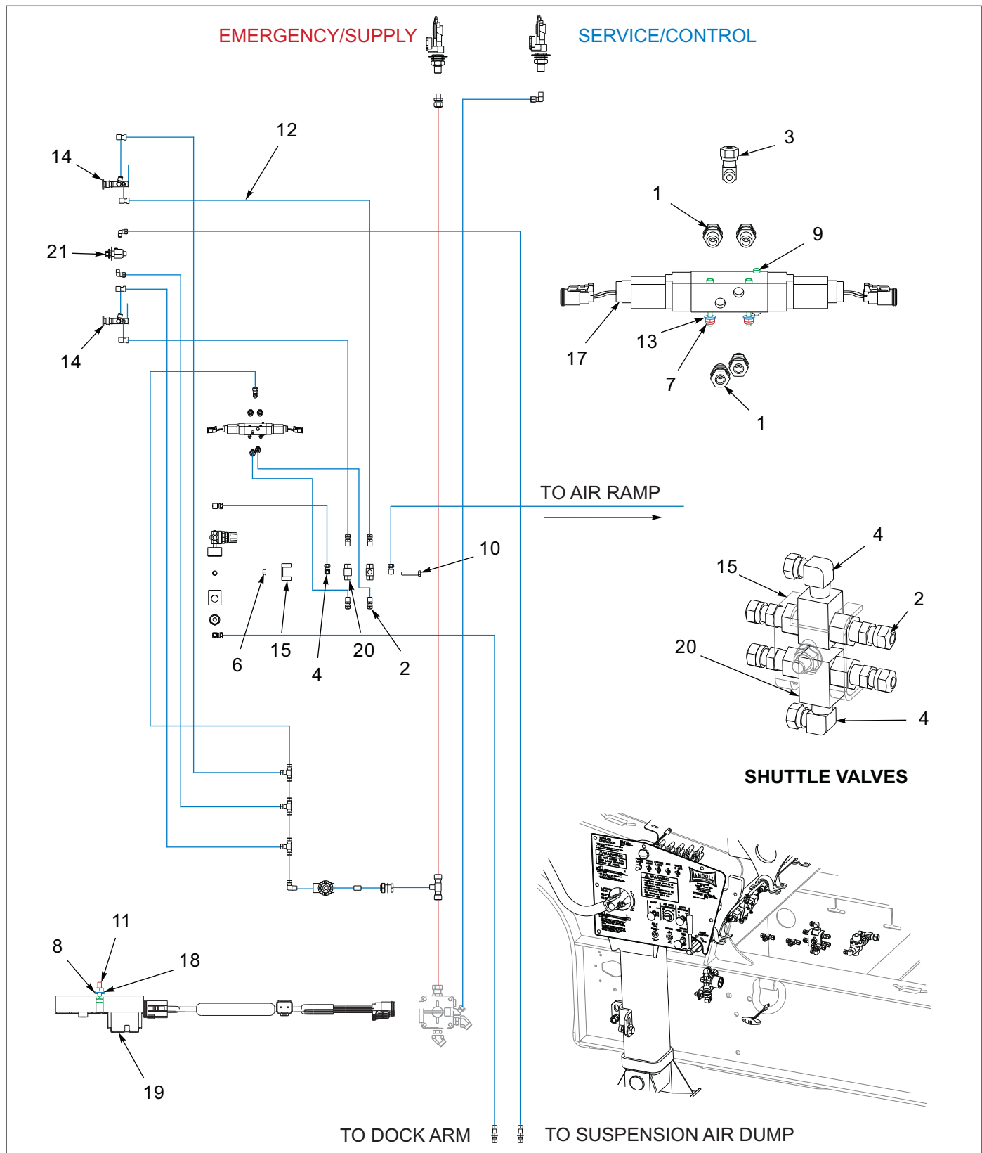
Figure 1-16: Remote Components
