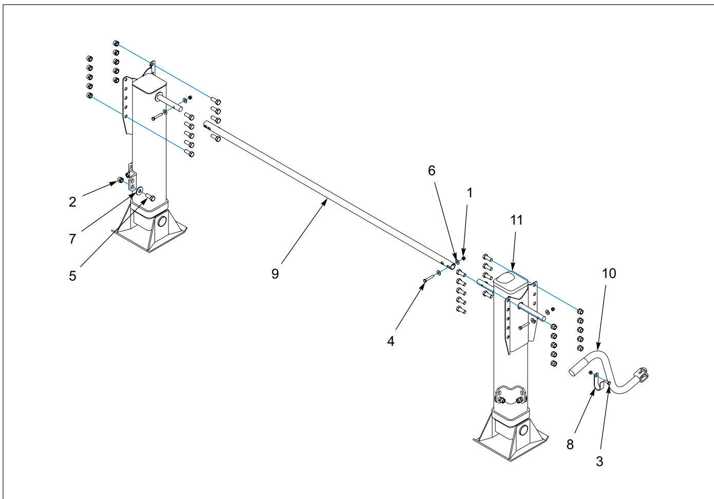
Figure 1-68: Jost 410
