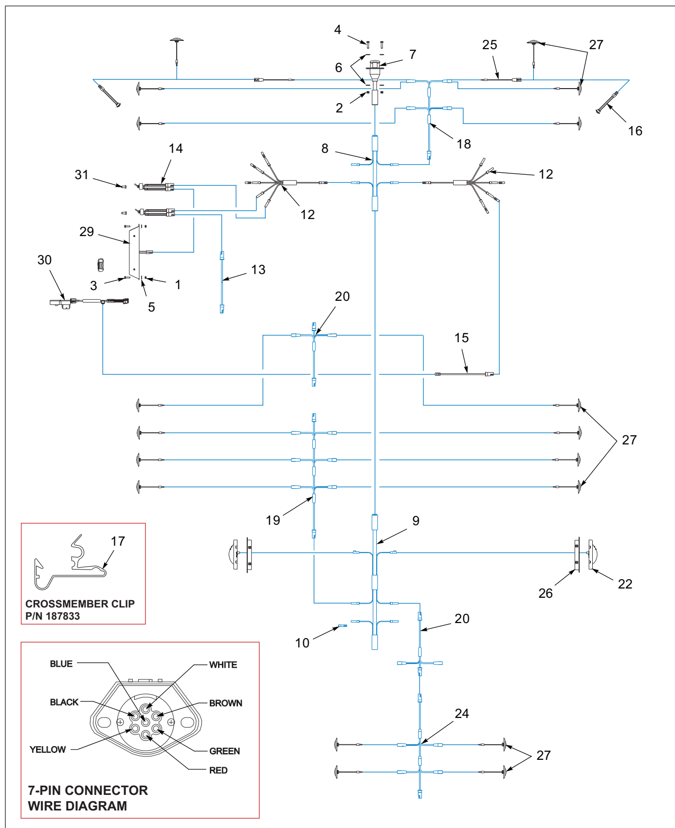
Figure 1-24: Electrical System (1 of 3)
