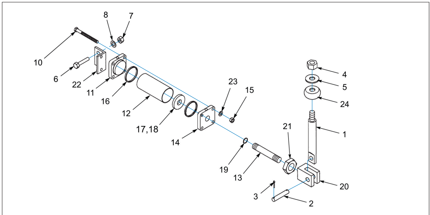
Figure 1-59: Winch - Air Shift Cylinder
