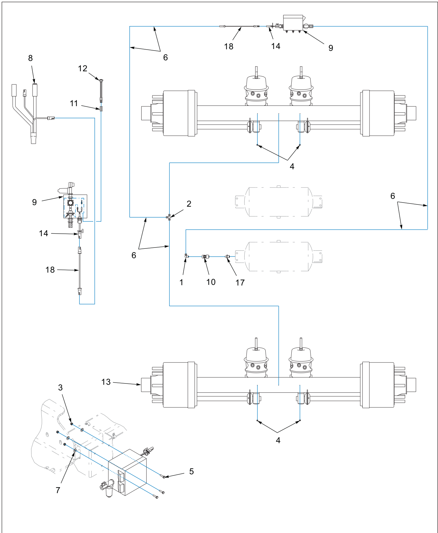
Figure 1-48: Tire Inflation System - 930E
