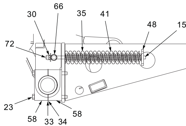
TAIL ASSEMBLY
