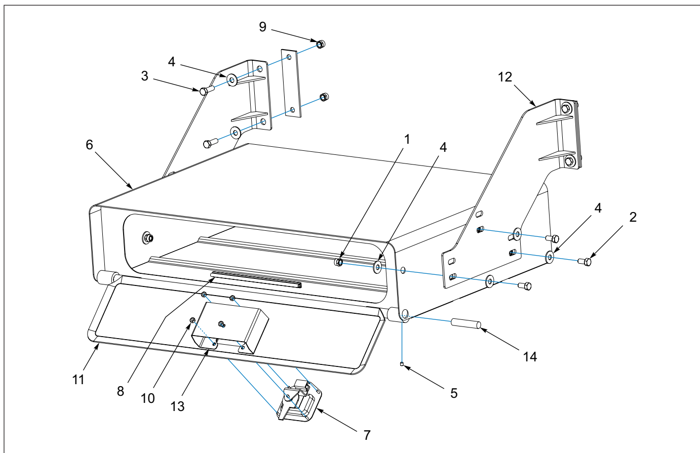
Figure 1-112: Toolbox Installation - Steel/Aluminum Door
