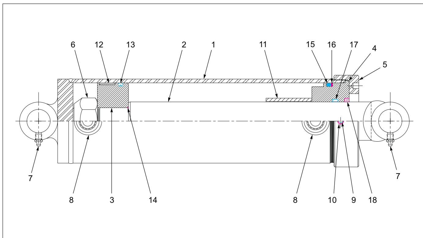
Figure 1-19: Cylinder - 5 X 60
