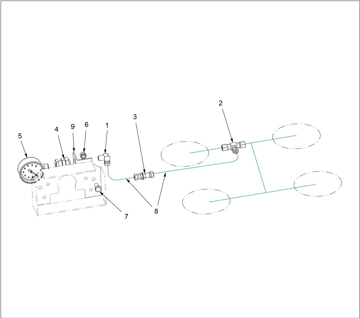
Figure 1-124: Pressure Gauge Installation
