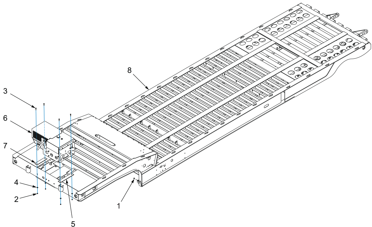
Figure 1-93: Mount Package W/O Winch
