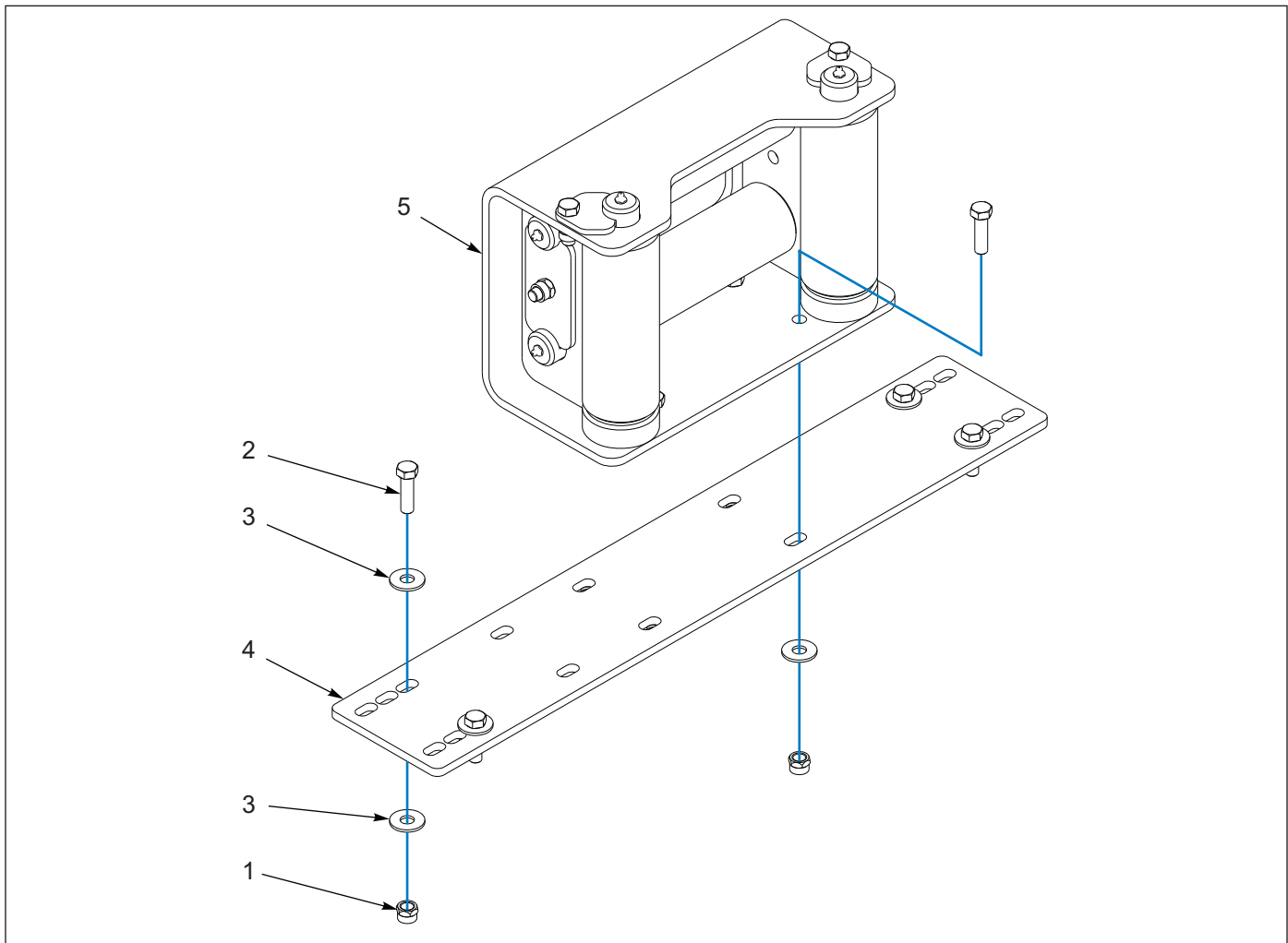
Figure 1-105: 4 Roller Guide Installation - 12K (BRADEN)
