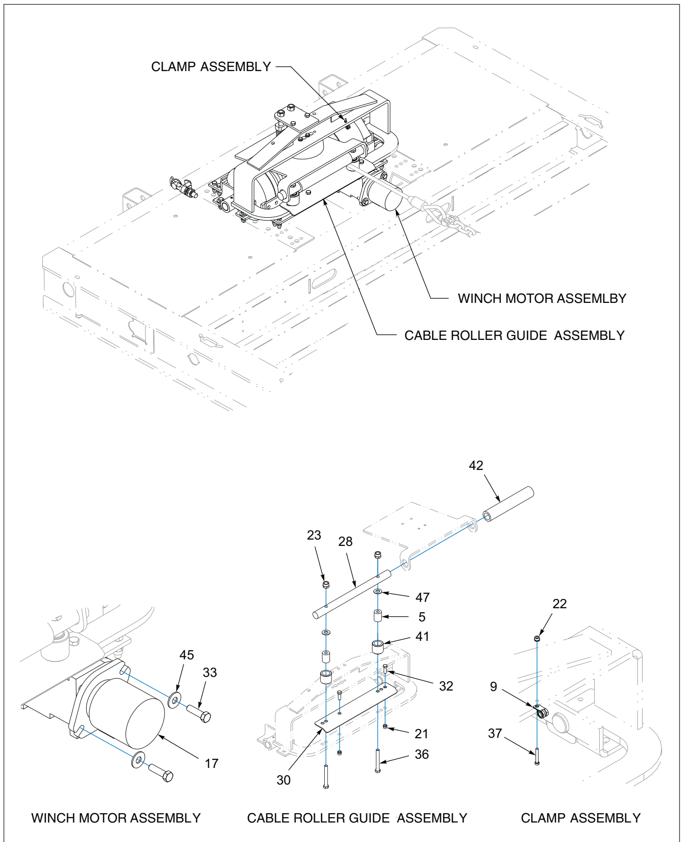
Figure 1-56: 20K Air Tension/Release (BRADEN) (2 of 3)
