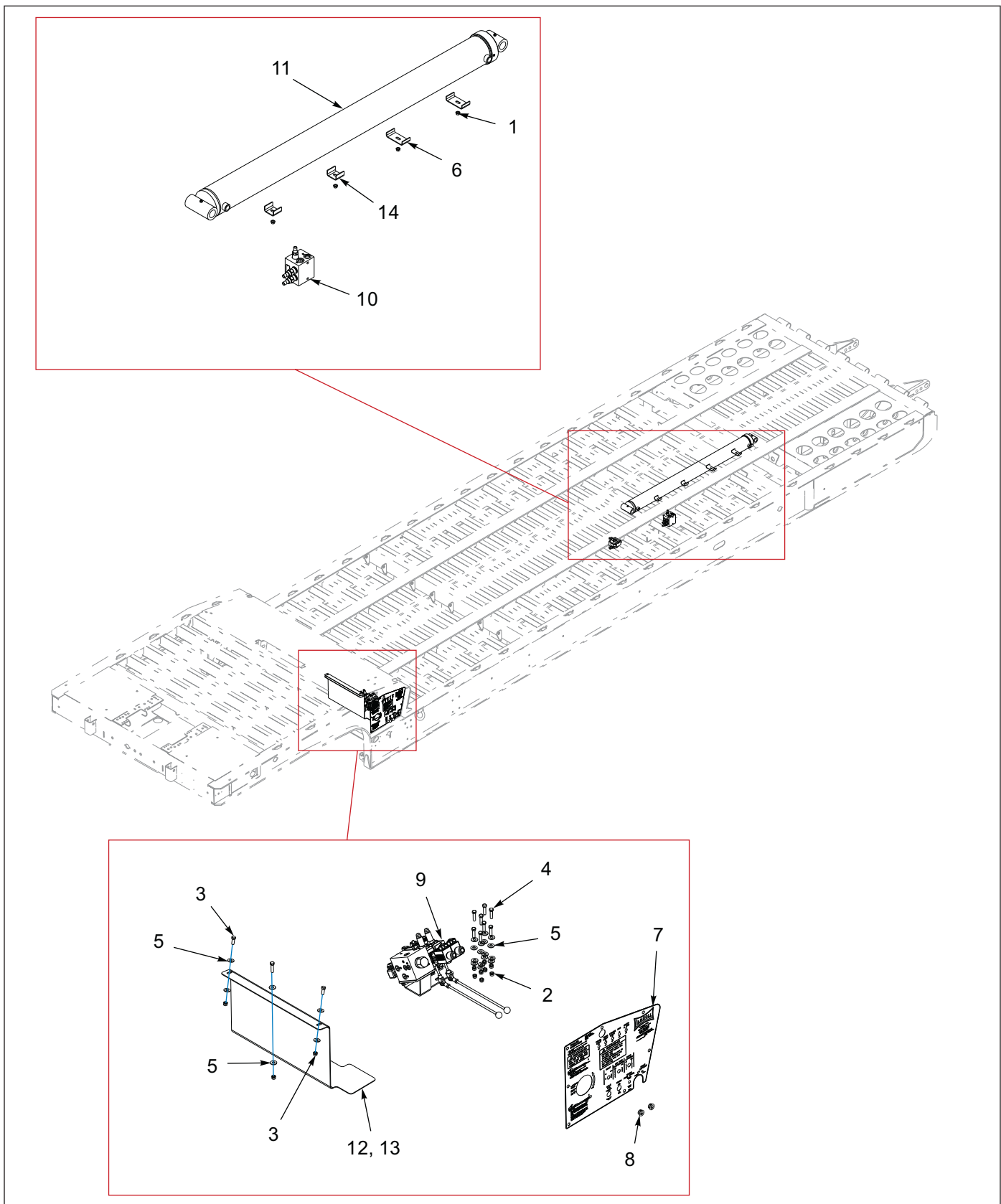
Figure 1-13: General Assembly - Hydraulic, Electric, Air
