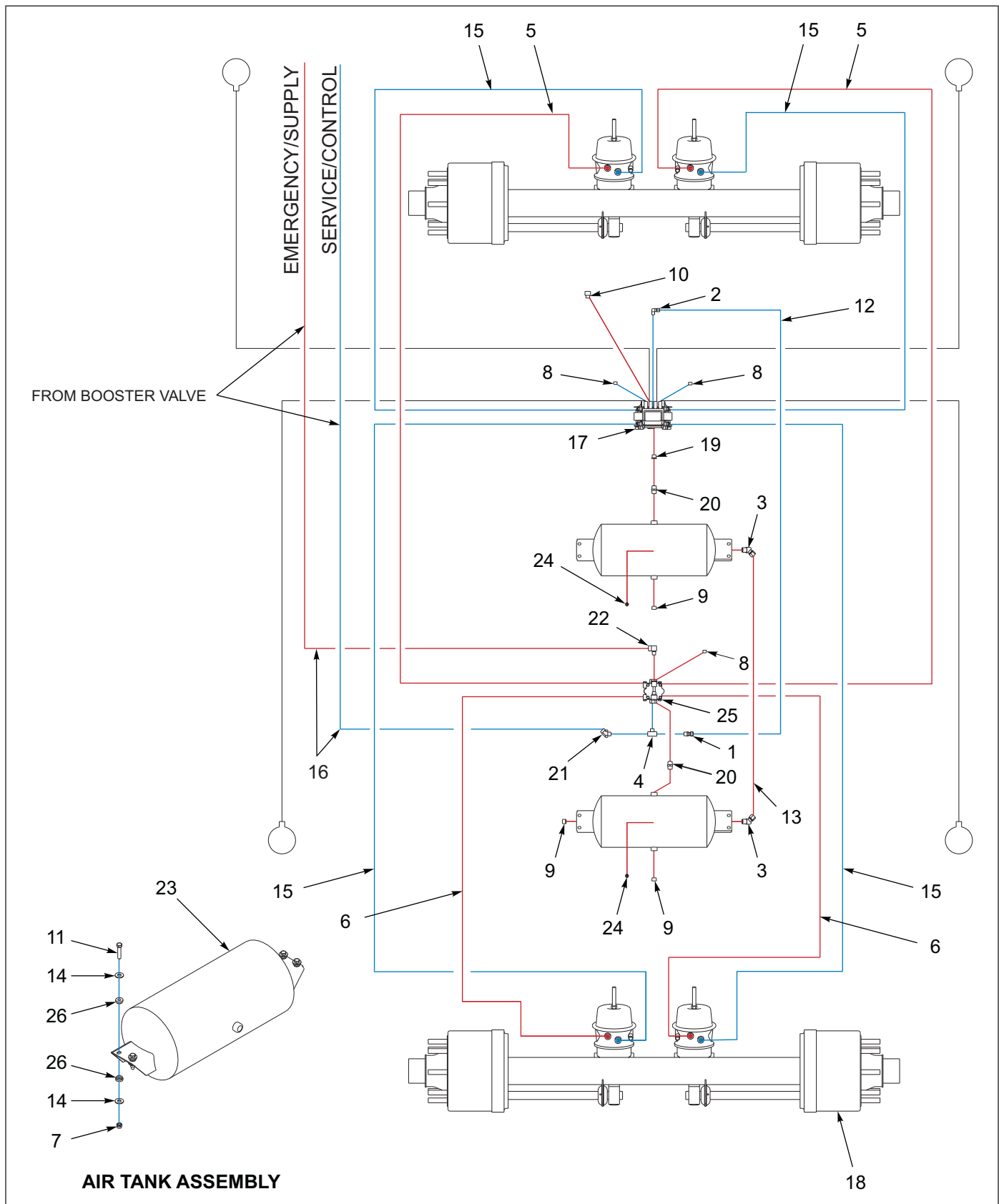
Figure 1-45: Air Brake System - 930E
