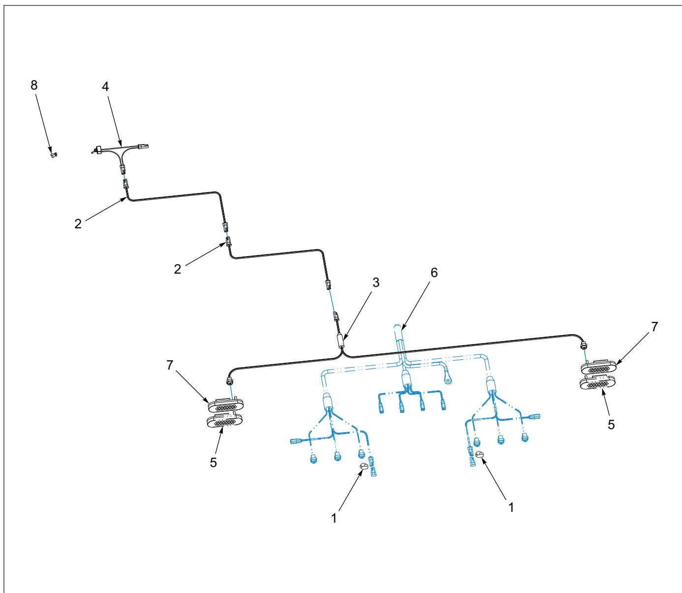
Figure 1-78: Strobe Installation
