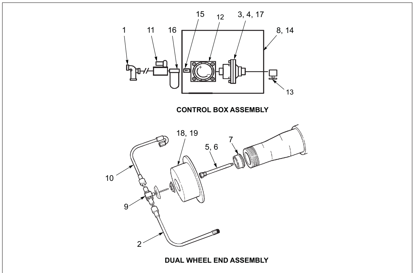
Figure 1-51: Tire Inflation System -Thermalert (3 SAF Axles)
