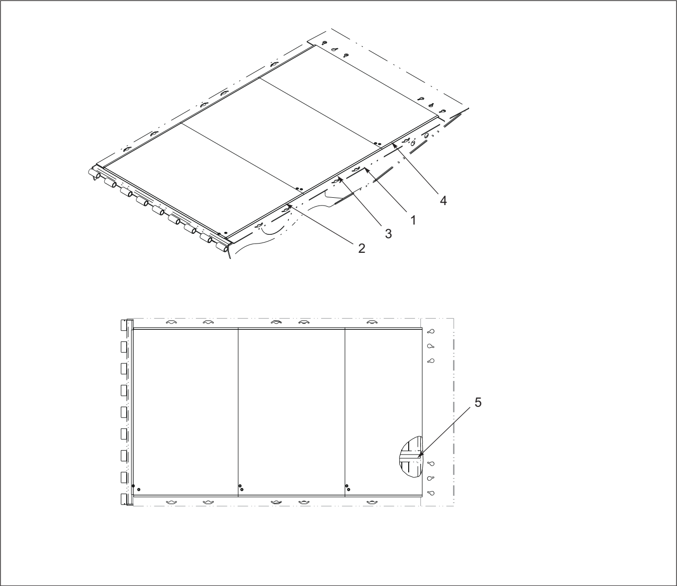
Figure 1-79: Deck Tread Grip/ Over Wood - 15' Tail
