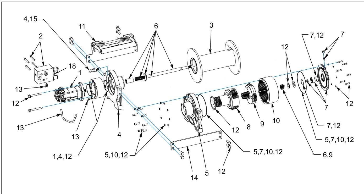
Figure 1-64: Winch Items - 20K 2 Speed (WARN)
