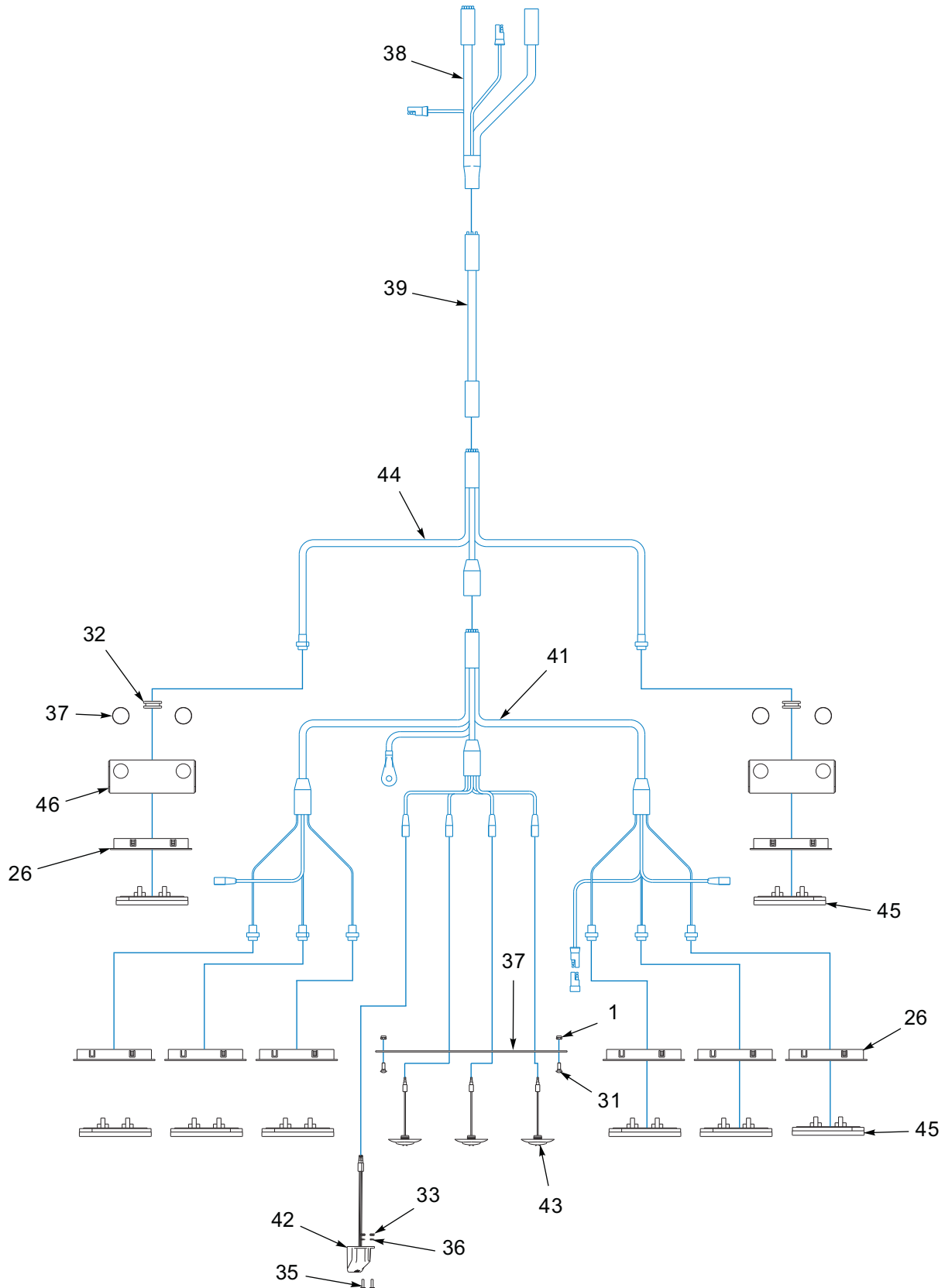
Figure 1-26: Electrical System (3 of 3)
