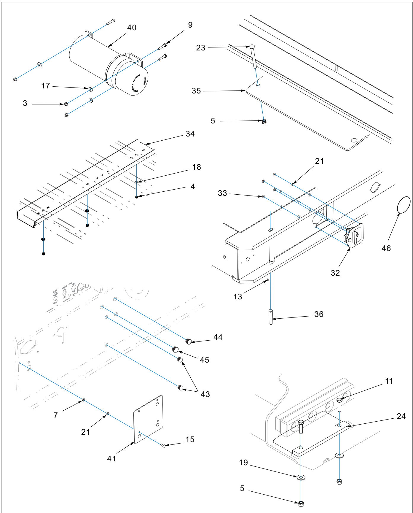
Figure 1-8: Frame Assembly (3 of 3)
