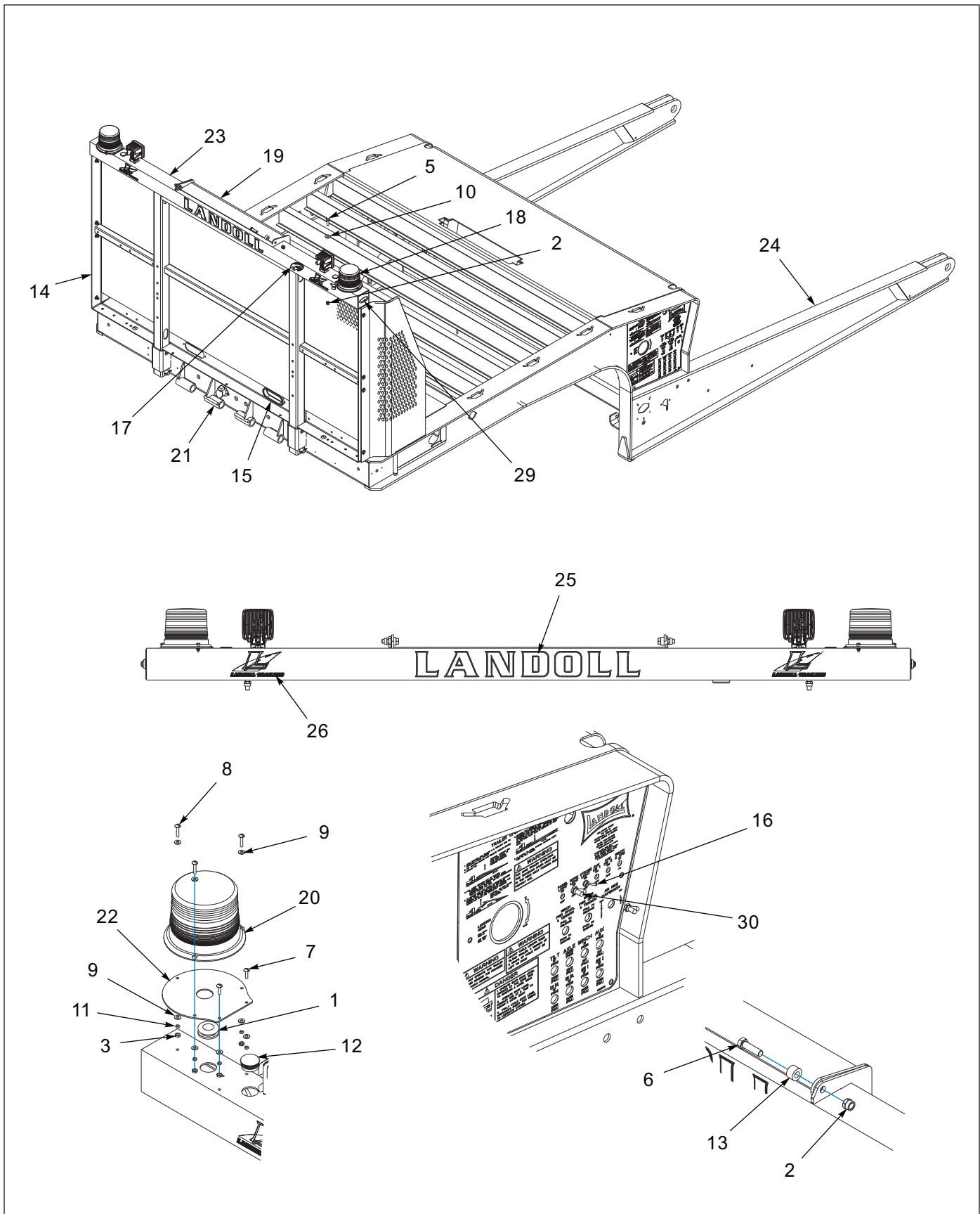
Figure 1-73: Chain Rack Lights General Assembly
