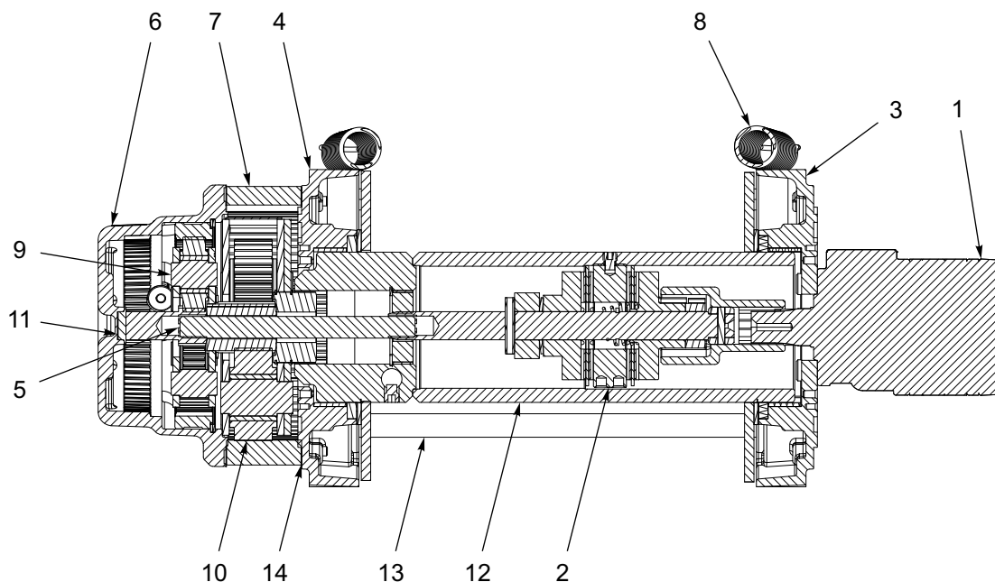
Figure 1-62: Winch Items - 12K (WARN)
