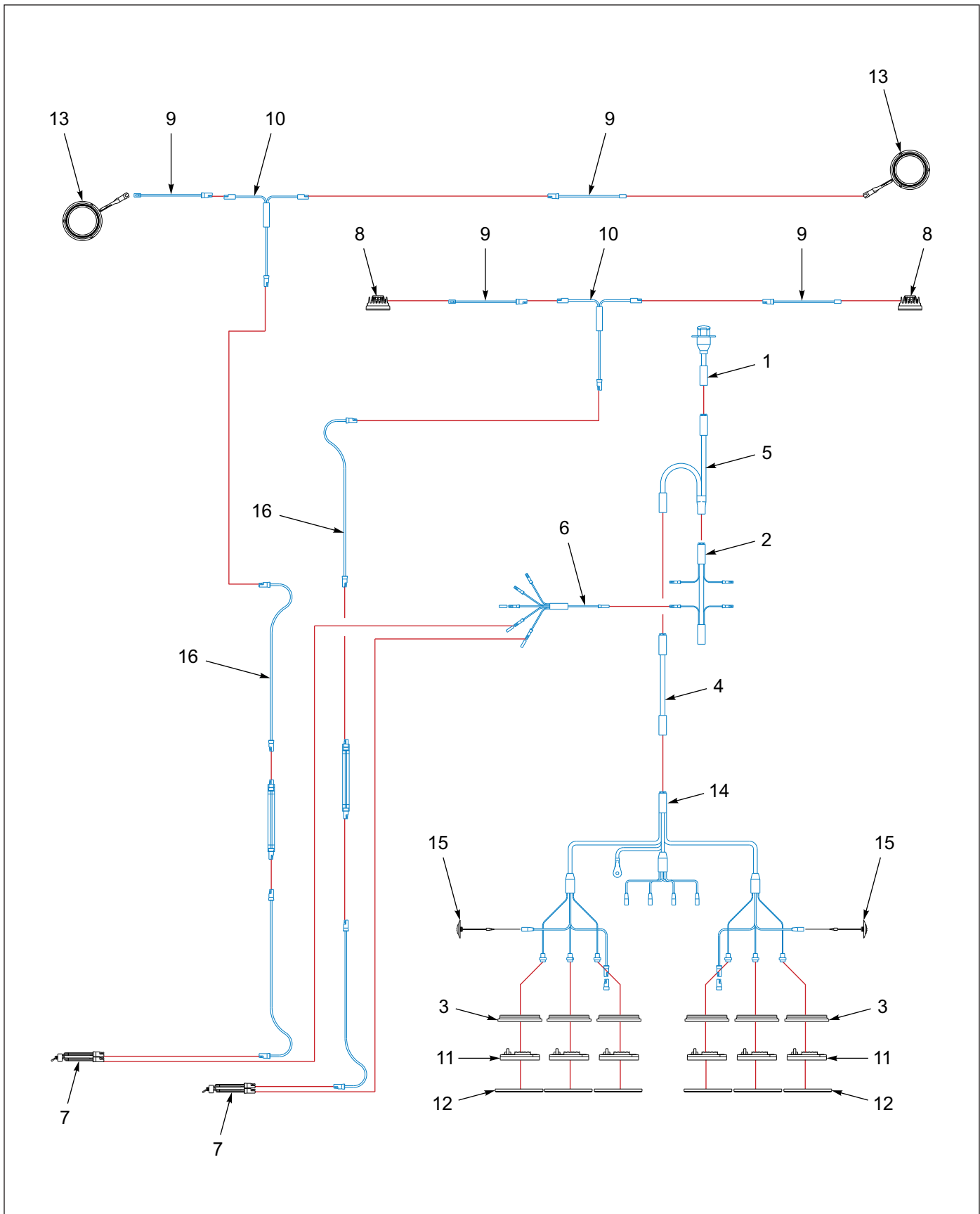
Figure 1-74: Chain Rack Lights Electrical System
