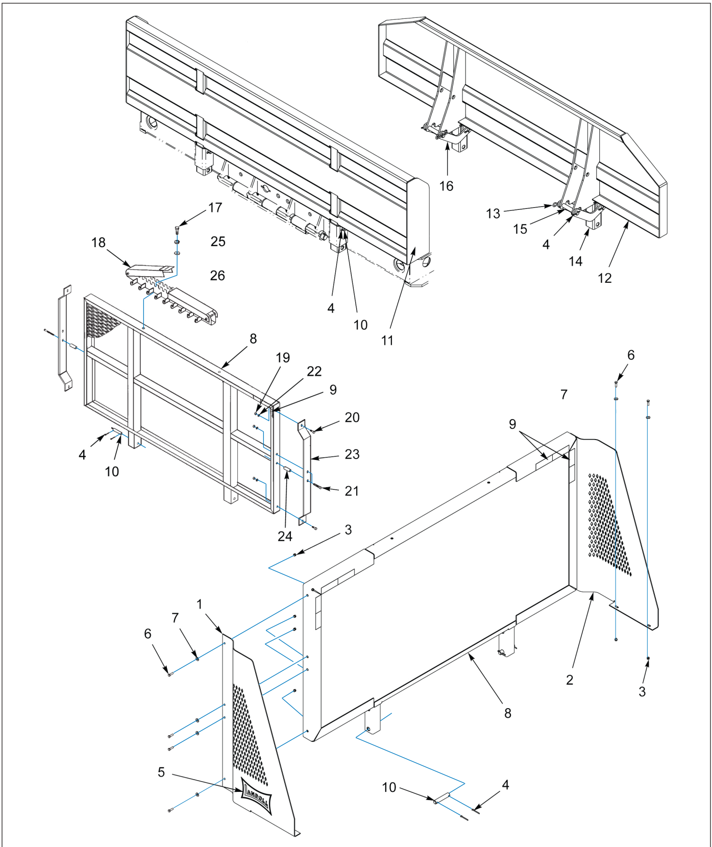
Figure 1-72: Bulkhead Assembly
