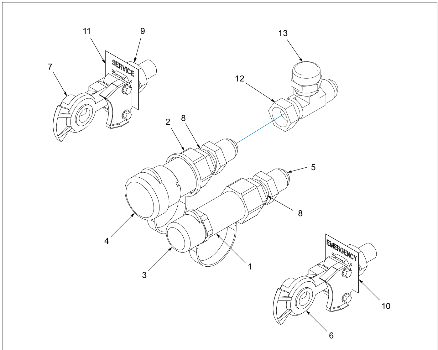
Figure 1-20: Connectors - Front Sub Assembly
