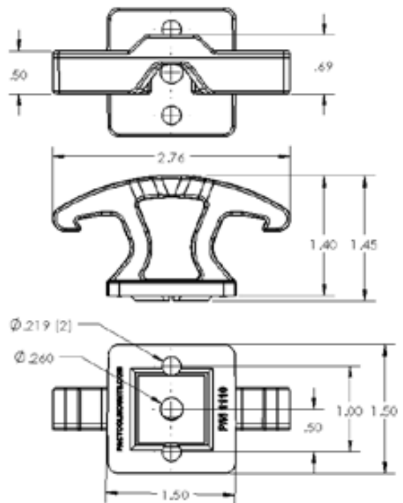
Dimensions: 1.45" x 1.5" x 2.76"
