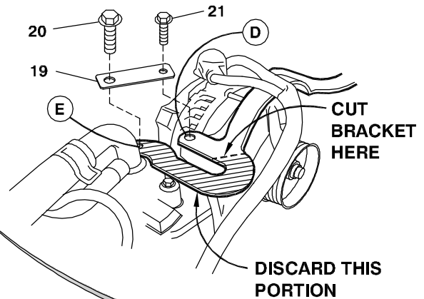
FIG. 4 MODIFY ALTERNATOR BRACKET 2009
